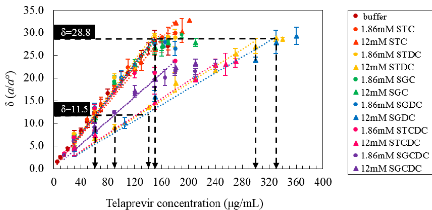
Figure 2. Telaprevir concentrations under constant supersaturation levels in the absence and presence of bile salts. The mass flow rate data from our previous study were used for determination of telaprevir supersaturation level in solutions containing different bile salts. 24
