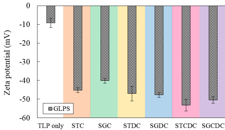
Figure 10. Zeta potential of highly supersaturated telaprevir solution in the absence and presence of 1.86mM bile salts.
