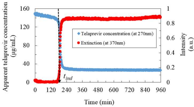
Figure 3. Crystallization induction time of a supersaturated telaprevir solution was determined as the time when a sudden increase in extinction signal and a sudden decrease in apparent concentration was observed.
