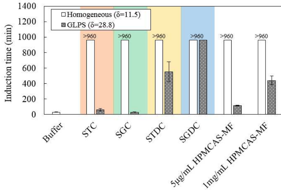
Figure 13. Induction time for telaprevir in the absence and presence of predissolved bile salts (at 1.86mM concentration) and the polymer, HPMCAS-MF (at 5µg/mL and 1mg/mL concentration).
