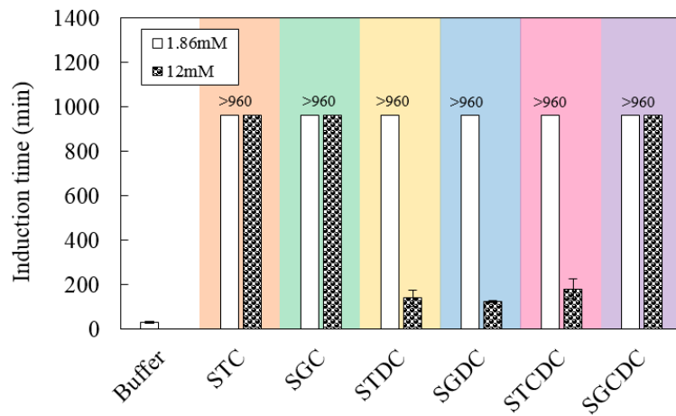
Figure 4. Induction time for telaprevir at supersaturation level of \delta=11.5 , in the absence and presence of predissolved 1.86mM and 12mM bile salts.
