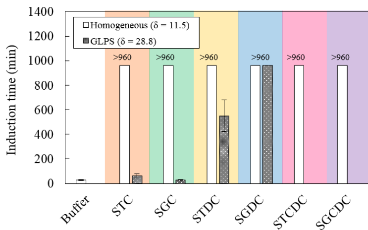
Figure 8. Induction time for telaprevir in the absence and presence of predissolved 1.86mM bile salts. Homogeneous solutions are at a concentration below the amorphous solubility of telaprevir, while GLPS refers to solutions just above the amorphous solubility of telaprevir which contain small ( \sim 300\text{nm} ) 42 amorphous telaprevir particles. Induction time results for solutions containing STCDC and SGDC at \delta=28.8 were not reported as the same supersaturation level cannot be reached due to partitioning of these two bile salts into telaprevir-rich phase. 24
