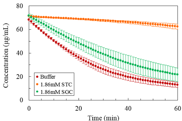
Figure 11. Desupersaturation profile of seeded telaprevir solution in the absence and presence of 1.86mM STC, and 1.86mM SGC. The slope of the initial desupersaturation profiles ( t < 10\text{min} ) was used to determine the mass growth rate.
