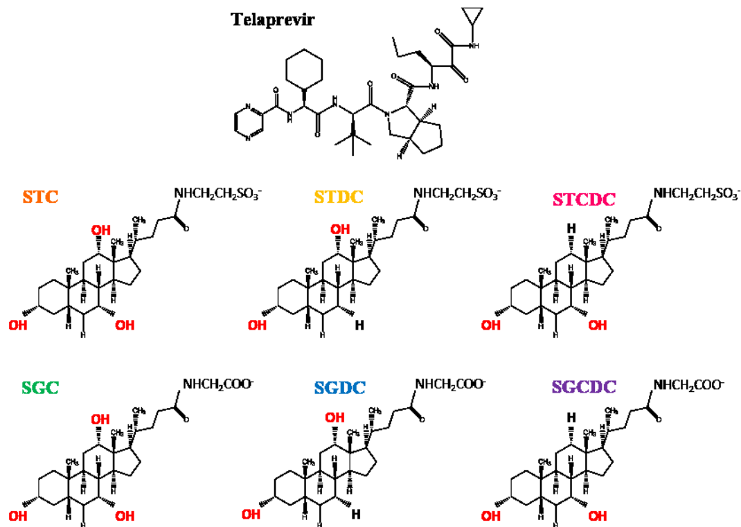
Figure 1. Molecular structures of telaprevir and bile salts.
