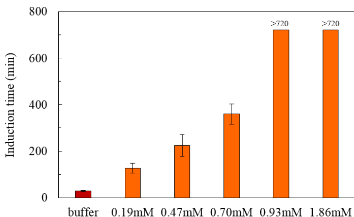
Figure 7. Effect of STC concentration on induction time with 60 \mu g/mL telaprevir ( \delta=11.5 ).
