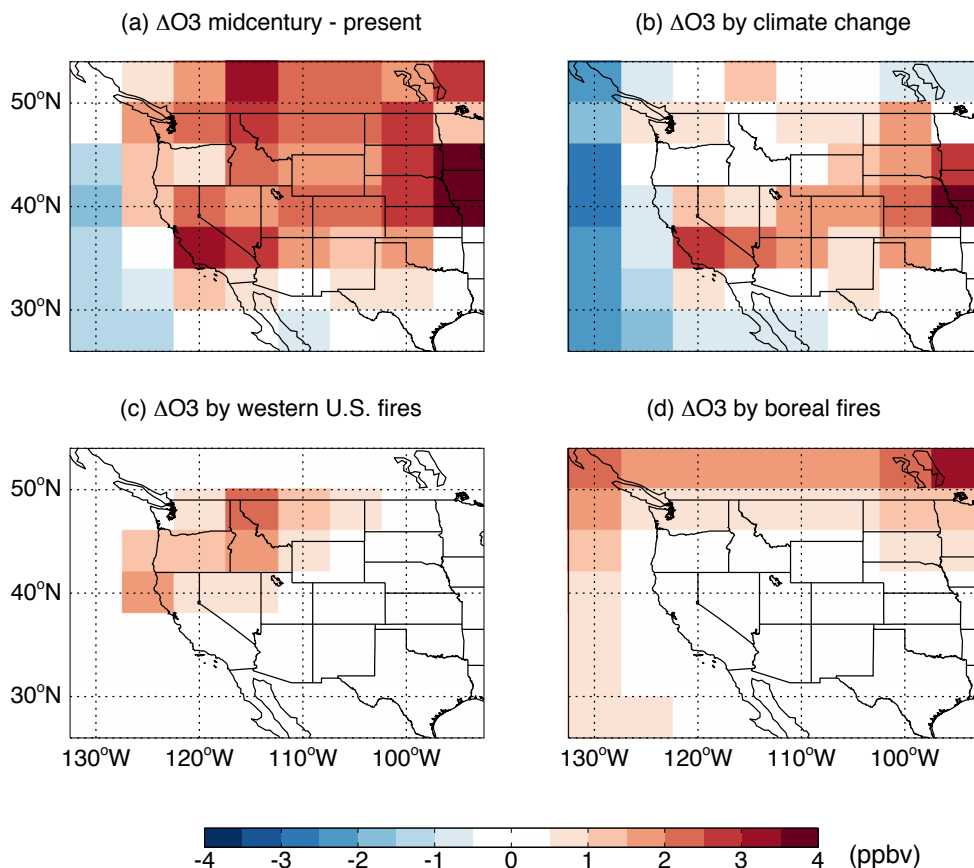
Figure 10. (a) Simulated changes in MDA8 ozone at the surface in summer (June–August) at the mid-century relative to the present day (FULL_A1B – FULL_PD) over the western and central United States. The other three panels show the contributions to the changes in (a) from (b) climate change (CLIM_CHAN – FULL_PD), (c) changes in fire emissions in the western US (FULL_A1B – BOREAL_FIRE), and (d) changes in fire emissions in Alaska and Canada (FULL_A1B – WUS_FIRE). Descriptions of the sensitivity simulations are given in Table 1.
