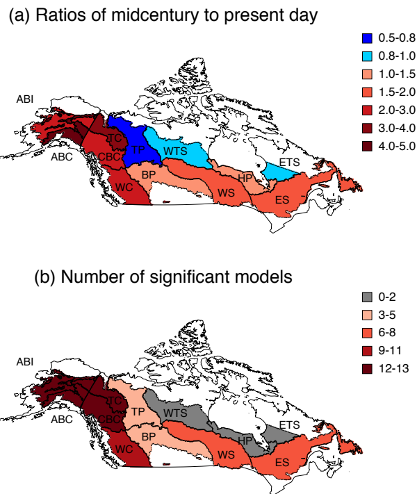
Figure 7. (a) Median ratios of mid-century (2048–2064) to present-day (1983–1999) area burned in each boreal ecoregion, as predicted by an ensemble of GCMs and (b) the number of GCMs out of 13 total which predict significant changes of the same sign as the median. The ecoregions are: Alaska Boreal Interior (ABI), Alaska Boreal Cordillera (ABC), Taiga Cordillera (TC), Canadian Boreal Cordillera (CBC), Western Cordillera (WC), Taiga Plain (TP), Boreal Plain (BP), Western Taiga Shield (WTS), Eastern Taiga Shield (ETS), Hudson Plain (HP), Western Mixed Wood Shield (WS), and Eastern Mixed Wood Shield (ES).
