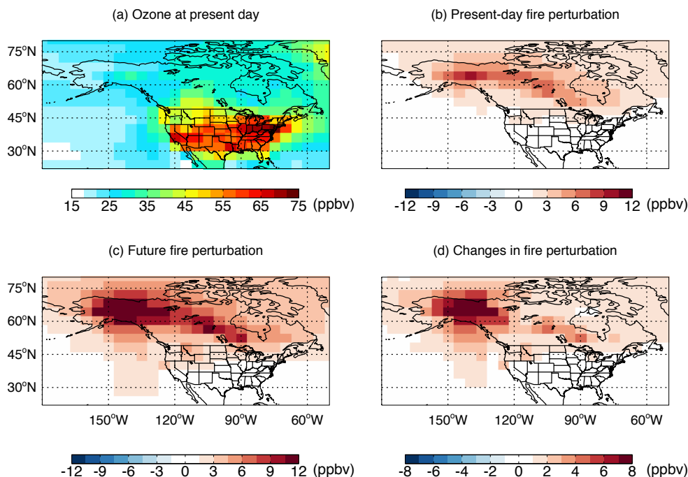
Figure 9. (a) Simulated present-day MDA8 ozone at the surface in summer (June–August). (b) shows the contribution to MDA8 summertime ozone by wildfire emissions in the present day (FULL_PD – NOFIRE_PD), and (c) shows the same contribution, but at the mid-century (FULL_A1B – NOFIRE_A1B). (d) presents the change in the contribution of wildfires to MDA8 ozone between the two periods (i.e., c–b). Descriptions of the sensitivity simulations are given in Table 1. The color scale saturates at both ends.
