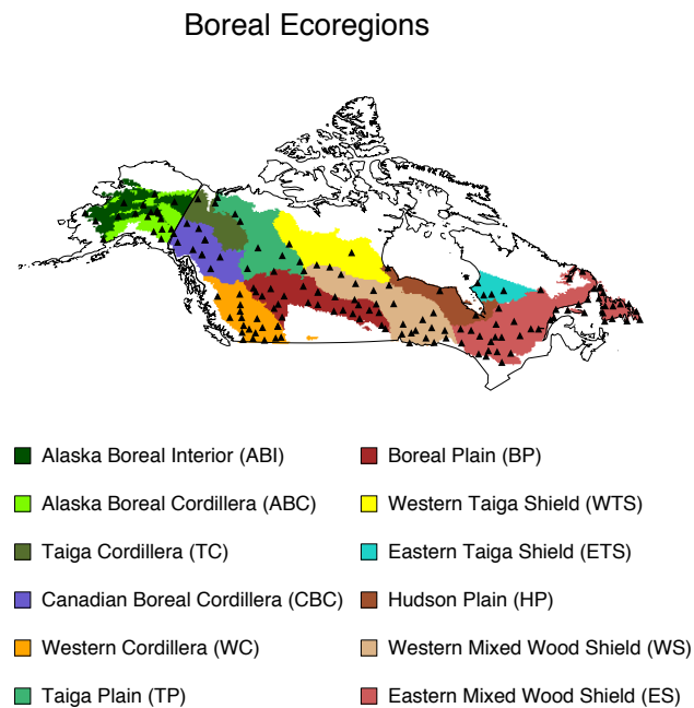
Figure 1. Distribution of the 12 ecoregions used for this study. The black triangle symbols indicate the GSOD meteorological data sites in Alaskan and Canadian ecoregions.
