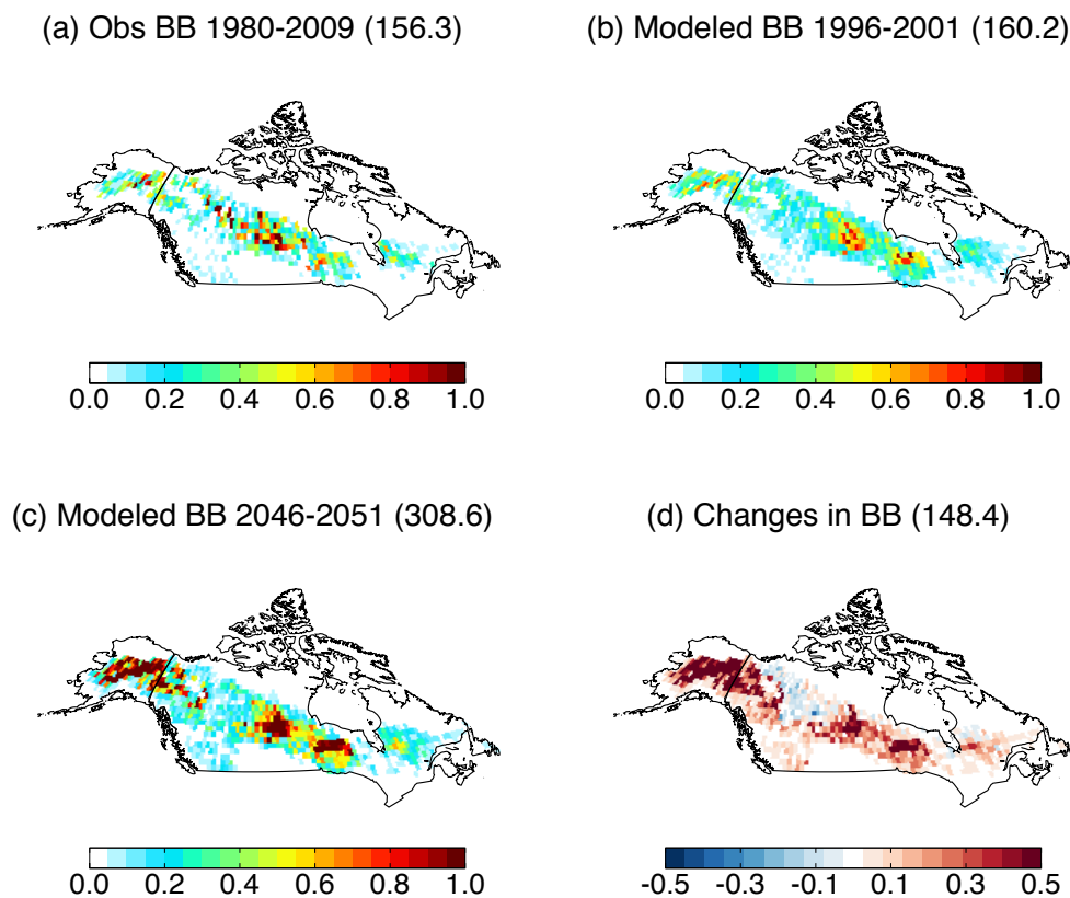
Figure 8. Biomass burning (BB) in Alaska and Canada in terms of dry matter (DM) burned per year, calculated as the product of area burned and fuel consumption. (a) shows values based on observations for 1980–2009, (b) the predicted values for 1996–2001, and (c) the projections for 2046–2051. The differences between mid-century and present day (c–b) are shown in (d). Annual mean values summed over the whole domain are shown in brackets. Units: Tg DM yr -1 .
