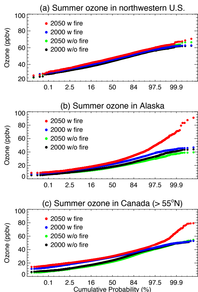
Figure 11. Simulated cumulative probability distributions of MDA8 ozone at the surface in summer (June–August) over (a) northwestern US ( >40^\circ\text{N} ), (b) Alaska, and (c) Canada ( >55^\circ\text{N} ) for different scenarios. Black shows the present-day (1997–2001) climate without wildfire emissions; green shows future (2047–2051) climate without wildfire emissions; blue indicates present-day climate including the associated wildfire emissions; and red indicates future climate including the associated wildfire emissions. Each point represents the value in one grid square within each region for each day during the five model summers (1997–2001 or 2047–2051).
