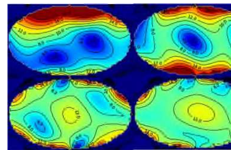
Fig. 6 Simulated B_1 -fields for using the first (top left), first two (top right), four (bottom left) and seven (bottom right) most efficient mode(s) of a 16-element MRI coil for RF-shimming.
