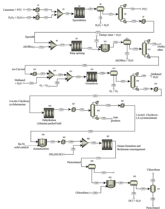
Figure 4. The proposed process flowsheet detailing all reaction and separation steps. The ASPEN flowsheet is shown for illustration only. All simulations were performed using gPROMS.
