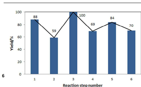
Figure 5. Yields of the individual reaction steps, corresponding to the flowsheet shown in Figure 4.
