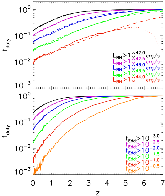
Figure 12. Top: redshift evolution of black hole duty cycle (solid lines; as in Fig. 11), together with our redshift-evolution fit from equation (8) [dashed lines]. Note that the fit is performed for 0 \leq z \leq 4 , but we plot a larger z -range to show behaviour at higher redshifts. The high-redshift decline for the L_{\text{BH}} > 10^{44} \text{ erg s}^{-1} population is due to the lack of sufficiently massive black holes capable of radiating at such high rates (with the imposed Eddington limit), represented by a dotted line. Bottom: redshift evolution for duty cycles of Eddington fraction-selected black hole populations, which eliminates the high-redshift decline.
