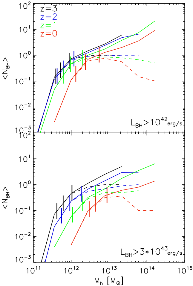
Figure 5. Mean occupation number of black holes above 10^{42} erg s^{-1} (top) and 3 \times 10^{43} erg s^{-1} (bottom). Solid lines show full black hole population; dashed lines show central black holes only. Vertical lines mark the host mass scale above which 90 per cent, 75 per cent and 50 per cent of black holes are found. Despite the lower occupation number, most black holes are found in the more common low-mass haloes, and high-mass haloes ( M_h \gtrsim 10^{12.5} - 10^{13} M_\odot ) tend to have significant numbers of satellite black holes.
