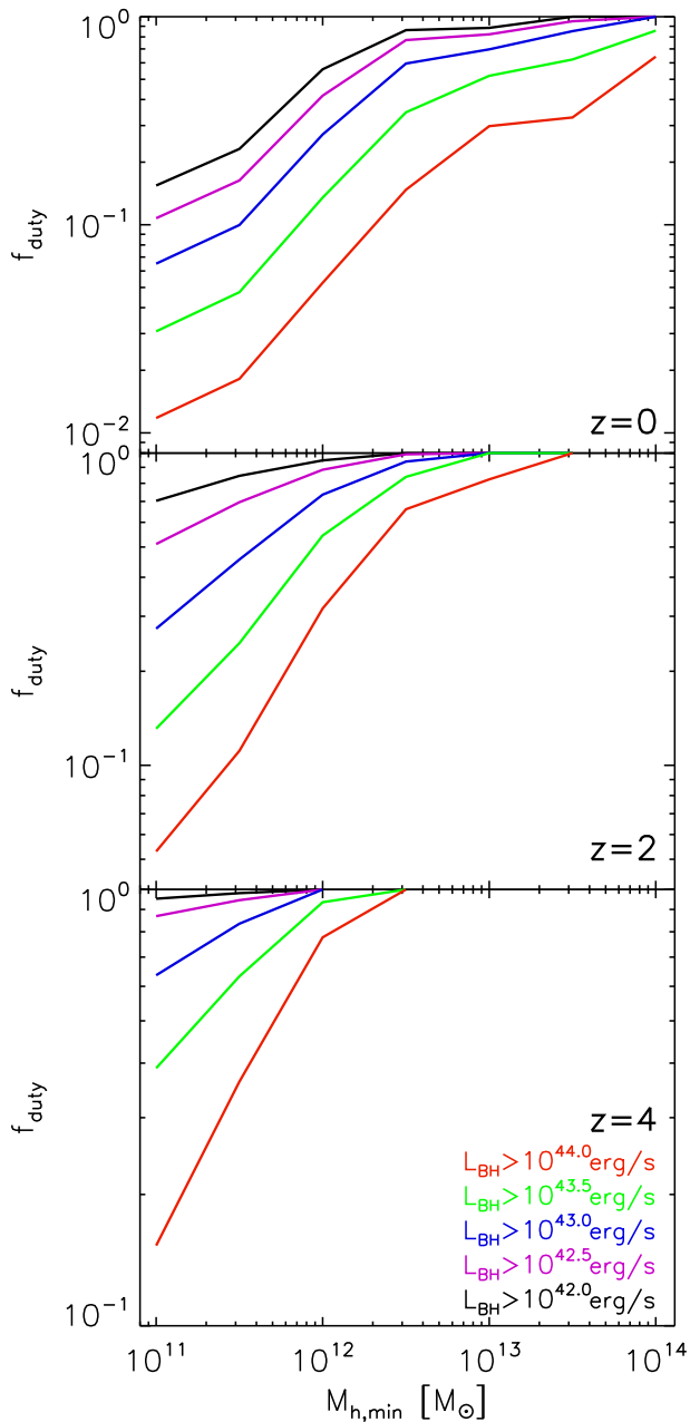
Figure 10. Duty cycle for haloes above a given luminosity (line colour) as a function of minimum halo mass, for z = 0, 2 and 4 (top, middle, bottom). Note that the y-axis range evolves with redshift, matching the range spanned by our simulation.
