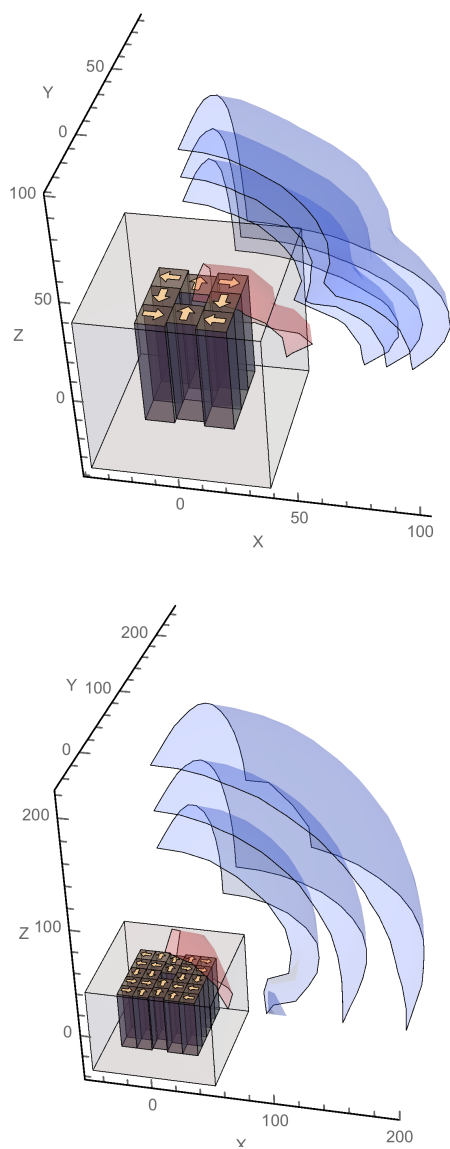
Figure 5: Calculated stray fields for the 8-block and 24-block magnet arrays (upper and lower plots, respectively). The contour surfaces represent field strengths of 5, 10, 20 gauss (in blue) and 1000 gauss (in red).
