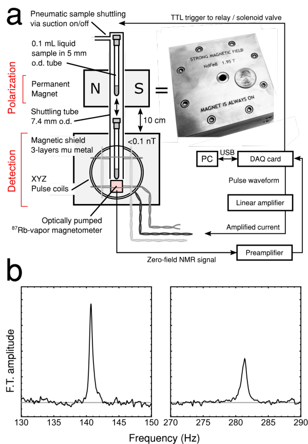
Figure 6: Experiment used to test the performance of the permanent magnet array for spin polarization in an NMR sample. Part (a) shows a schematic view of a home-built zero-field NMR spectrometer based on an optically pumped rubidium magnetometer. The sample, contained in a standard 5 mm NMR tube, is polarized within the permanent magnet and then shuttled into a magnetic shield where the magnetometer resides. After transport to zero field, a DC pulse excites the spin coherence and the signal is detected by the magnetometer. In (b) we show the spectrum recorded for 0.1 mL neat ^{13}\text{C} -methanol, where the signals appear at 1\times and 2\times the scalar ^1J_{\text{CH}} coupling frequency.
