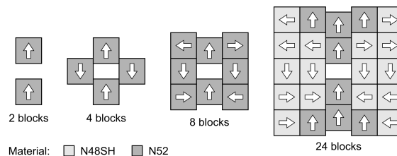
Figure 1: Cross sections of the Pseudo-Halbach permanent magnet assemblies involving 2, 4, 8 and 24 NdFeB magnet blocks. Arrows represent the axis of magnetization in the material. The first three structures use a single type of material, while the last one uses two types to reduce demagnetization effects.
