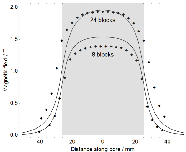
Figure 4: Field strengths of the 8-block and 24-block magnet arrays versus distance along the bore axis. The diamonds correspond to experimental measurements using a Hall-effect probe, while the solid lines correspond to the result of advanced numerical modeling of the magnet array, given the materials data provided (see Supplementary Information).
