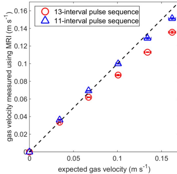
Fig 3. Measurements of the vertical component of SF 6 gas velocity through a packed bed (i.e. no fluidization) of poppy seeds ( d_p = 1.1 mm). The measurements give the average gas velocity over the cross-section of the bed at a height 50 mm above the distributor. Measurements were made using (◐) the Cotts 13-interval pulse sequence [20], which is widely regarded as the best existing MRI technique for measuring flow in heterogeneous systems, and (◔) the newly-developed 11-interval pulse sequence [28]. All measurements were repeated 3 times and showed a standard deviation of less than 0.002 m/s. Measurements were compared with the expected velocity, given by the dotted black line and calculated as U/\varepsilon , where \varepsilon is the void fraction. The superficial velocity U was calculated from gas flow meter measurements. Uncertainty for the expected gas velocity, as given by the horizontal error bars, arises from the uncertainty in the void fraction measurement. Parameters for the measurements are shown in Table 3.
