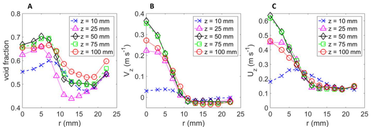
Fig. 7. MRI measurements of time-averaged (A) void fraction, (B) vertical particle velocity and (C) vertical gas velocity as a function of radial position at different heights ( z ) above the distributor; expanded bed height: 120 mm.
