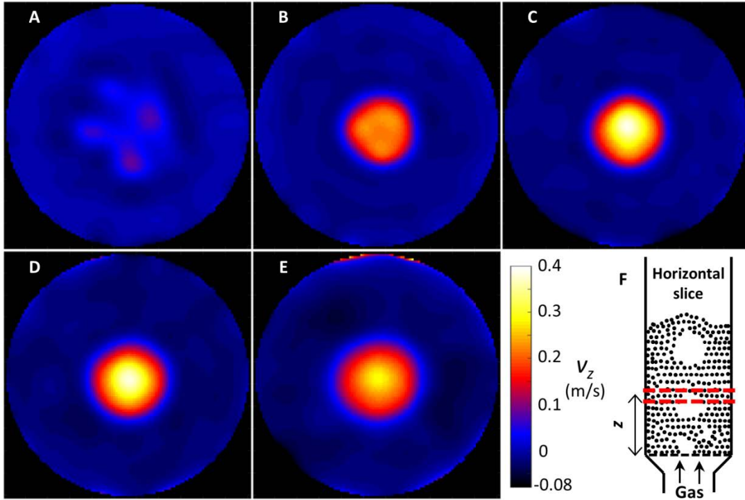
Fig. 5 Time-averaged particle velocity maps of poppy seeds at different vertical positions in the fluidized bed. Fluidization regime: bubbling; U = 0.104 m/s; field-of-view: 53 mm ( x ) by 53 mm ( y ); FWHM slice thickness: 4 mm ( z ); pixel size: 0.47 mm ( x ) by 0.47 mm ( y ); vertical positions above distributor: (A) z = 10 mm, (B) z = 25 mm, (C) z = 50 mm, (D) z = 75 mm, (E) z = 100 mm; expanded bed height: 120 mm.
