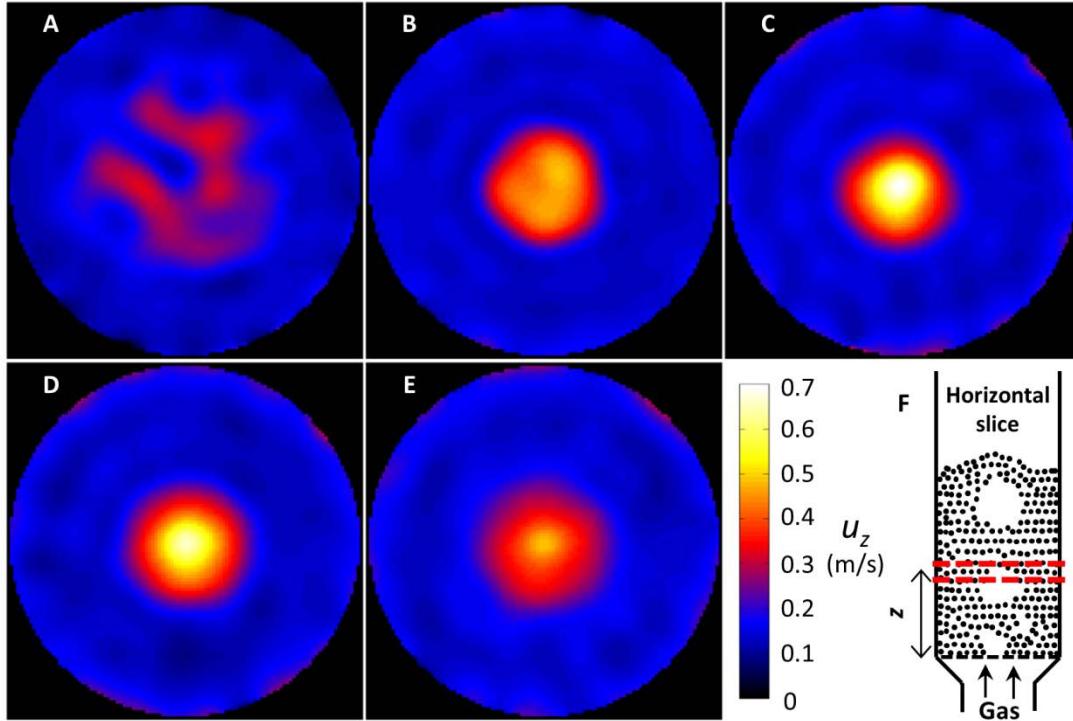
Fig. 6 Maps of time-averaged gas velocity of \text{SF}_6 at different vertical positions in the fluidized bed. Fluidization regime: bubbling; U = 0.104 m/s; field-of-view: 53 mm ( x ) by 53 mm ( y ); FWHM slice thickness: 4 mm ( z ); pixel size: 0.47 mm ( x ) by 0.47 mm ( y ); vertical positions above distributor: (A) z = 10 mm, (B) z = 25 mm, (C) z = 50 mm, (D) z = 75 mm, (E) z = 100 mm; expanded bed height: 120 mm.
