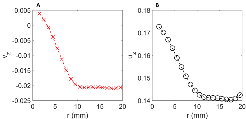
Fig. A1. Particle velocity (A) and gas velocity (B) in the emulsion region for the experimental data as a function of radius used for the cutoff between the bubbling and emulsion regions.
