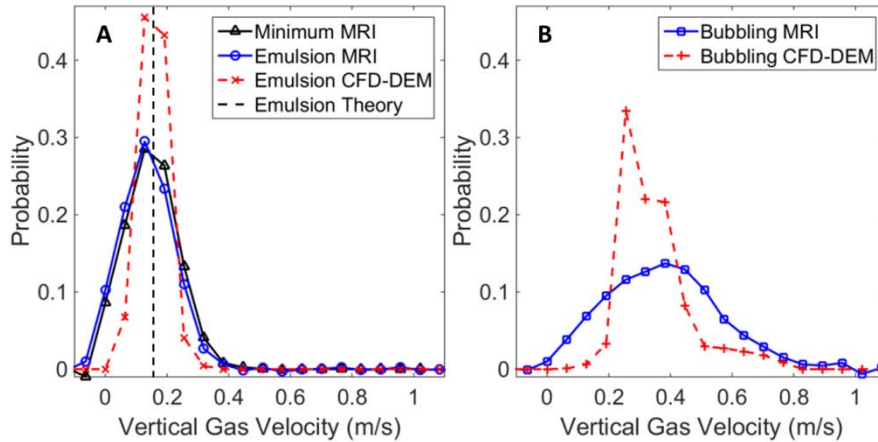
Fig 9. Probability distribution functions of vertical gas velocity in (A) the emulsion region and (B) the bubbling region (regions shown in Fig. 8). MRI measurements were compared with CFD-DEM predictions. In (A), comparison is also given with MRI measurement of velocity distribution across the entire cross-section at minimum fluidization, and the vertical dashed line gives the prediction of analytical theory (Eq. 8) [9,44] for gas velocity in the emulsion region.
