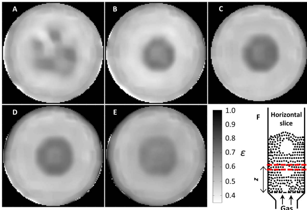
Fig. 4 Time-averaged void fraction maps obtained from intensity maps of poppy seeds at different vertical positions in the fluidized bed. Fluidization regime: bubbling; U = 0.104 m/s; field-of-view: 53 mm ( x ) by 53 mm ( y ); FWHM slice thickness: 4 mm ( z ); pixel size: 0.47 mm ( x ) by 0.47 mm ( y ); vertical positions above distributor: (A) z = 10 mm, (B) z = 25 mm, (C) z = 50 mm, (D) z = 75 mm, (E) z = 100 mm; expanded bed height: 120 mm.
