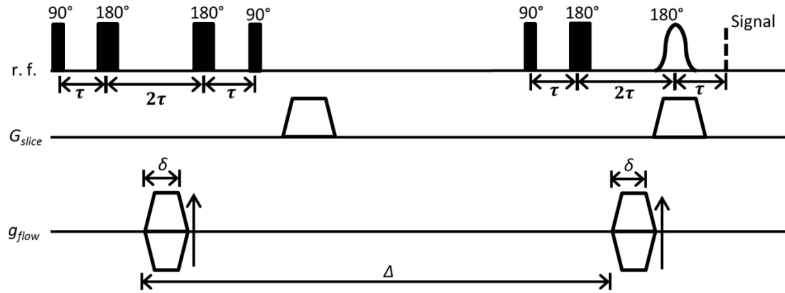
Fig. 1. Pulse sequence diagram for 11-interval MRI velocimetry.
