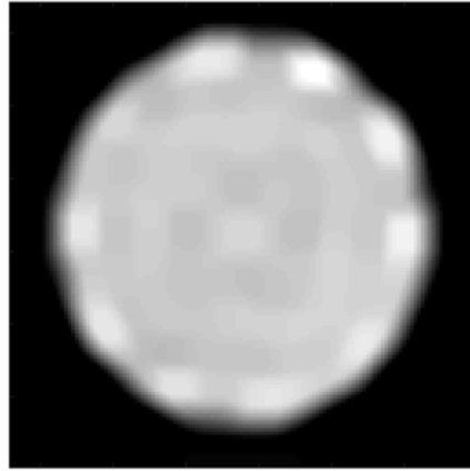
Fig. 2 Map of signal intensity arising from oil in poppy seeds in packed bed used to calibrate void fraction in fluidized bed measurements with white regions indicating high signal intensity and black regions indicating zero signal. Field of view 60 mm (x) by 60 mm (y); slice thickness: 4 mm, z = 50 mm above distributor; pixel size: 0.47 mm (x) by 0.47 mm (y).
