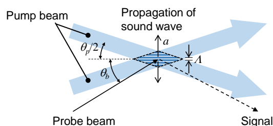
Fig. 1 Schematic of LITGS. Here, \theta_p is incident angle of the pump beams and \theta_b is the Bragg angle.
