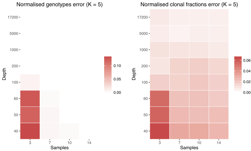
FIG. 6. Reconstruction errors on validation data obtained running Cloe with K = 5 clones. The heatmaps show the genotypes error (left) and clonal fractions error (right) for various combinations of depth and samples.
