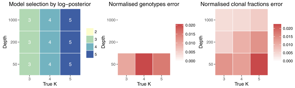
FIG. 4. Results on the simulated datasets. Left: inferred model size for every combination of K and depths. Centre and right: reconstruction errors. All datasets consisted of five samples and 100 mutations.
