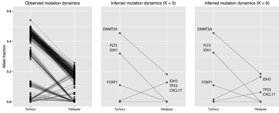
FIG. 10. Observed and inferred mutation dynamics for 257 mutations from the ALLDNA dataset; driver mutations are highlighted. Left: observed allele fractions; centre: predicted allele fractions given the parameters inferred by Cloe using 5 clones; right: predicted allele fractions given the parameters inferred by Cloe with 6 clones. The allele fraction predicted for a mutation j in a sample t is given by \frac{1}{2} \sum_k z_{jk} f_{kt} .
