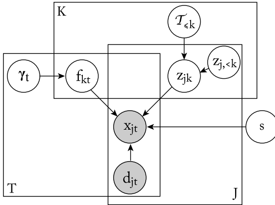
FIG. 3. The full graphical model of Cloe.
