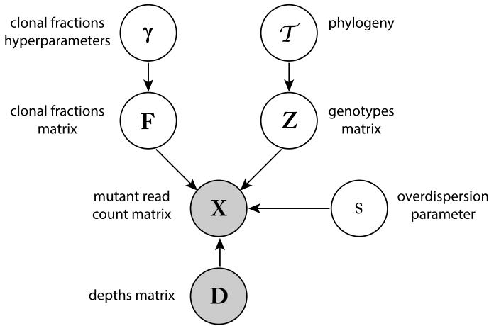
FIG. 2. Simplified graphical model corresponding to Cloe, omitting overlapping plates and convergent evolution relations.
