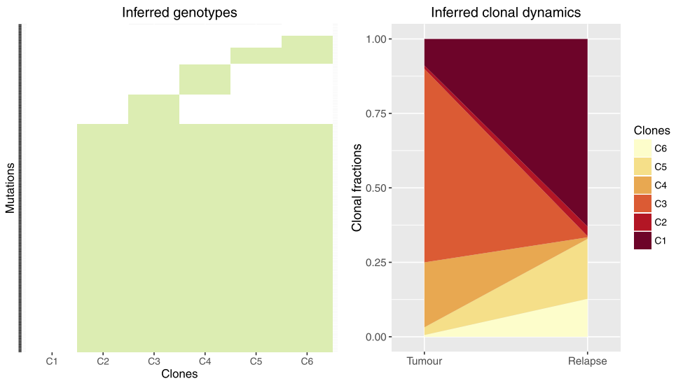
FIG. 11. Parameters inferred by Cloe running with 6 clones on 257 mutations from the ALLDNA dataset. Genotypes are shown on the left, where green denotes presence of a mutation; clonal fractions for each clone are shown on the right. C1 is fixed as the normal contamination. The corresponding phylogeny is shown in Supplementary Figure 20.
