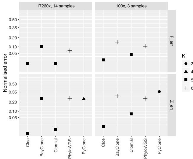
FIG. 7. Comparison of Cloe against four published methods on our validation dataset. Z_{err} denotes the reconstruction error on genotypes, and F_{err} the error on clonal fractions. The column headers denote the data that were analysed in each instance. The legend refers to the number of inferred clones; the correct number is five.
