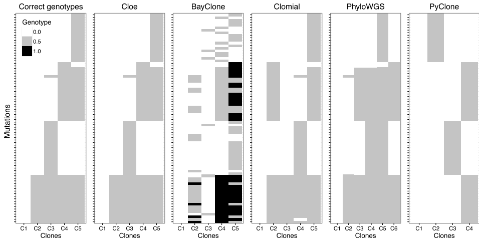
FIG. 8. Comparison of the genotypes inferred by the five benchmarked methods using all the data in our validation dataset. PyClone's reconstruction is a clustering of the mutations. In this representation, solutions were padded with the normal clone (C1) for a more direct comparison with our method. The legend refers to the proportion of mutated alleles out of two.
