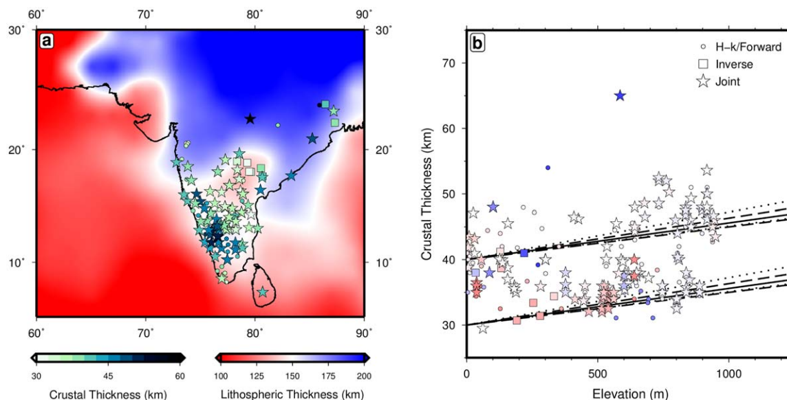
Figure 5. Crustal isostasy and lithospheric thickness. (a) Lithospheric thickness based upon surface wave tomographic model. Symbols are published crustal thickness estimates [Priestley and McKenzie, 2013] (Supporting Information Data Set S1). Stars = crustal thicknesses calculated by joint inversion of receiver functions and surface wave dispersion curves [e.g., Rai, 2003; Julià et al., 2009; Rai et al., 2009; Acton et al., 2010, 2011; Vijay Kumar et al., 2012; Mandal, 2012; Borah et al., 2014]; squares = crustal thicknesses from inverse modeling of receiver functions [e.g., Mitra et al., 2008; Kayal et al., 2011; Singh et al., 2012; Praveen Kumar and Mohan, 2014]; dots = crustal thicknesses calculated by either forward modeling or H-k stacks of receiver functions [e.g., Saul et al., 2000; Ravi Kumar et al., 2001; Gupta et al., 2003; Rai et al., 2005; Pathak et al., 2006; Tiwari et al., 2006; Jagadeesh and Rai, 2008; Rai et al., 2013]. (b) Crustal thickness plotted as function of elevation for different lithospheric thicknesses. Colored stars/squares/dots = crustal thicknesses calculated as before where color indicates lithospheric thickness at that location; solid lines = isostatic relationships determined by equalizing lithostatic pressure at base of either 30 or 40 km thick crust using crustal density of 2.7 Mg m -3 ; dashed lines = relationships calculated for crustal densities of 2.65 and 2.75 Mg m -3 ; dotted lines = relationships calculated for crustal densities of 2.76 and 2.9 Mg m -3 (i.e., density range estimated from v_p/v_s ratios) [Brocher, 2005].
