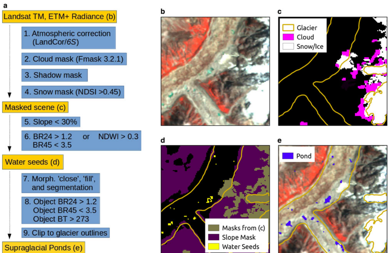
Fig. 3. (a) Processing workflow for supraglacial pond classification, with intermediate steps shown in insets (b)–(e). (b) Subset of Landsat TM false-color composite for 19 August 2009 after Landcor/6S processing. (c) Cloud, snow/ice and shadow (not shown) masks determined by subroutines, showing some difficulty with cloud identification. (d) Slope mask and determination of high-probability water seeds. (e) Pond cover output after image morphological operations and reclassification.
