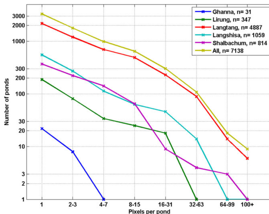
Fig. 5. Log/log plot of observed supraglacial pond size distribution for each glacier, 1999–2013. Each Landsat pixel covers 900 \text{ m}^2 .
