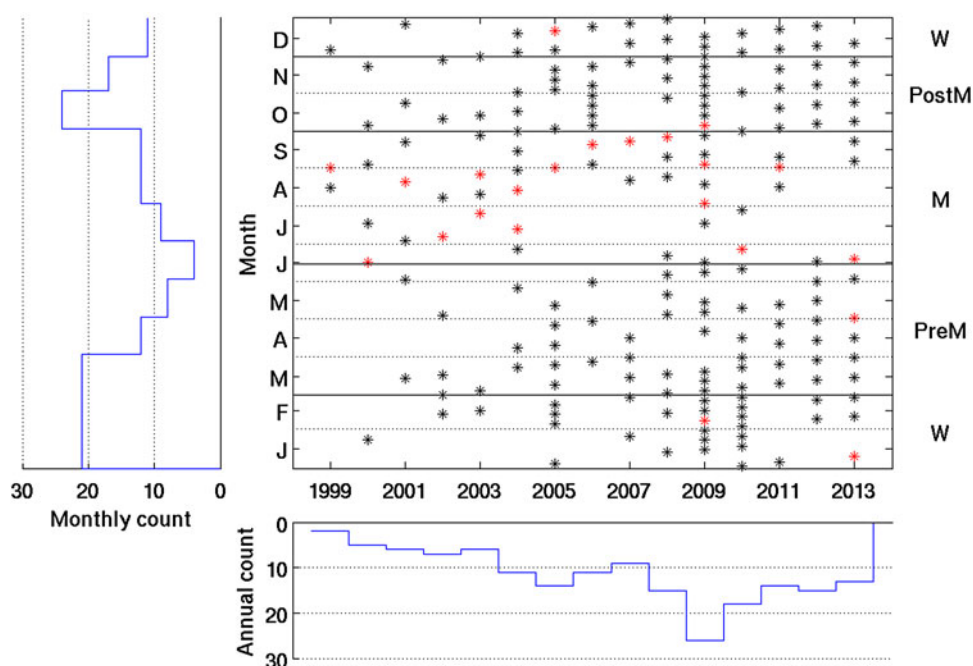
Fig. 2. Temporal distribution of scenes processed in the study, with histograms indicating monthly (left) and annual (bottom) counts of observations. Red marks are those scenes with < 50\% debris-covered area observable, which were removed from the analysis (26 removed from 198 scenes processed). Black marks are the scenes used in the analysis ( n = 172 ).
