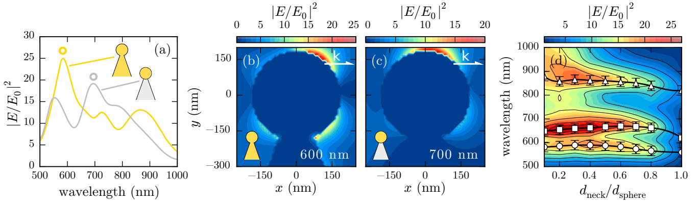
FIG. 4. (a) Numerically simulated near-field apex spectra of spherical Au and AuNP-on-Pt tips with (b,c) near-field maps of the main resonance in each, as highlighted by circles in (a). Simulated tips have a 300 nm spherical radii, 120 nm neck widths, 20^\circ opening angles and 1.88 \mu\text{m} lengths to best match typical experimental tip geometries and avoid truncation artefacts. Tips are illuminated by plane waves orientated along the tip axis. (d) Interpolated field enhancement map with superimposed resonant wavelengths, as the neck width varies from a spherical to a sharp tip. Tips have a 250 nm apex diameter, 1.88 \mu\text{m} length, and 10^\circ opening angle.
