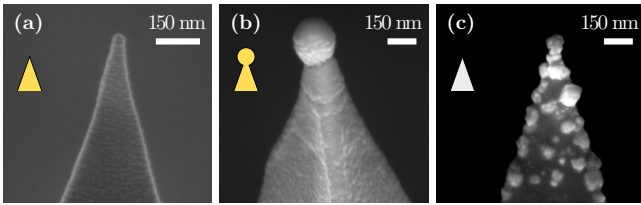
FIG. 2. SEM images of (a) sharp Au AFM tip, (b) Au-coated spherical AFM tip (Nanotools), and (c) electrochemically-deposited AuNP-on-Pt AFM tip.
