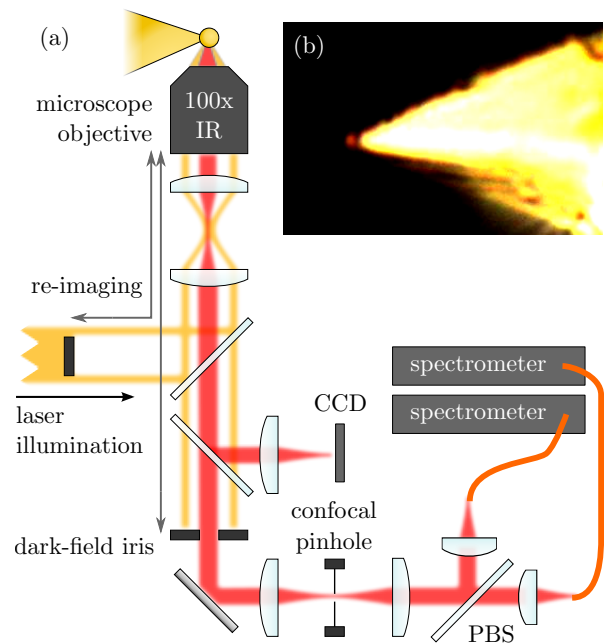
FIG. 1. (a) Hyperspectral imaging with supercontinuum laser focussed onto the tip apex for imaging, and the tip is raster scanned across the beam with scattering spectra of both polarisations acquired at each position. (b) Ball-tip imaged in dark-field microscopy.
