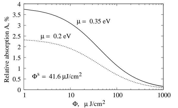
FIG. 3: Saturable optical absorption of a MoS 2 composite at E_\omega = 0.8 \text{ eV} . The parameters are the same as in Fig. 2. The saturation fluence is estimated from Eq. (23) with L \rightarrow L^{\text{eff}} , but Eq. (24) gives nearly the same result for \Phi^s of about 40 \mu\text{J}/\text{cm}^2 . It corresponds to the intensity of a few MW/cm 2 at the electron-hole recombination time of the order of 10 ps, see Ref. 41
