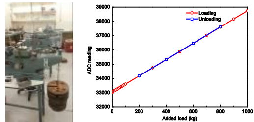
(a) Test apparatus (b) Test results Figure 3. Calibration on the load cell using direct shear apparatus: (a) Test apparatus; (b) Test results.
