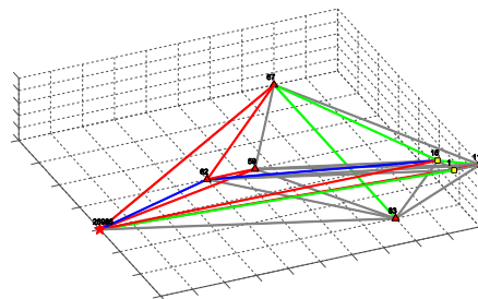
Figure 8. Network topology in Trinity Hall. Link colour represents the average number of connections made to the gateway per day
