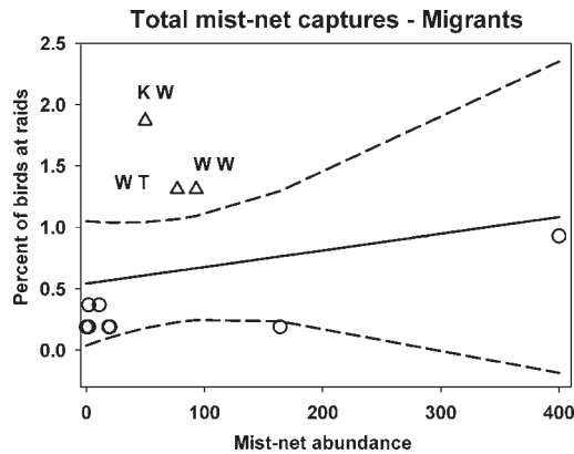
FIG. 2. Frequency of army ant raid attendance plotted against estimated local abundance for migrant bird species (Monteverde, Costa Rica). Solid line: linear regression best fit. Curved dashed lines: 95% confidence intervals (CI). Triangle symbols indicate species with raid attendance above the 95% CI (KW = Kentucky Warbler; WW = Wilson's Warbler; WT = Wood Thrush).
