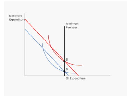
Figure 8b: Optimal response given binding minimum purchase amount
