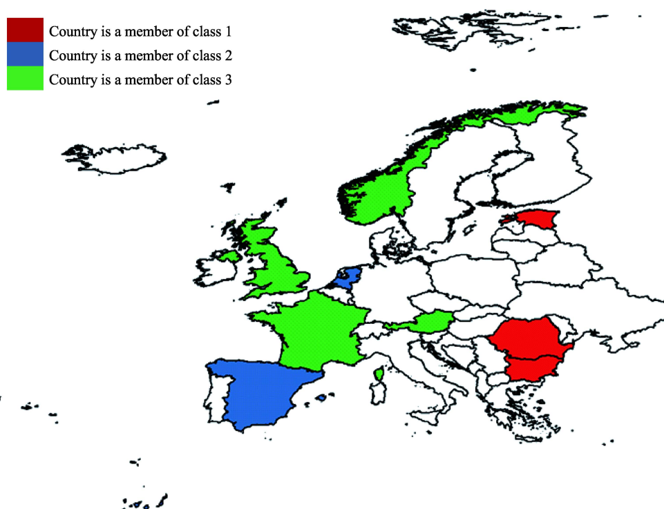
Figure 2. Allocation of countries to latent classes.
