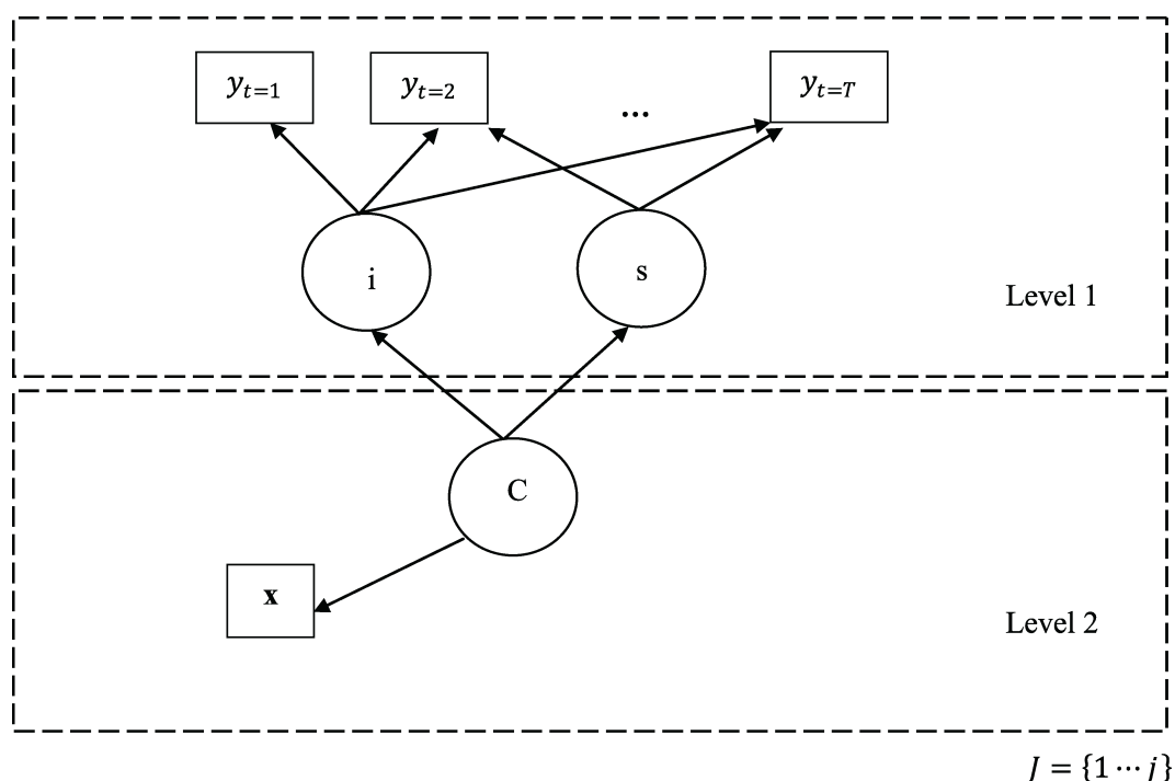
Figure 1. Structural equation representation of two level latent class models employed.
