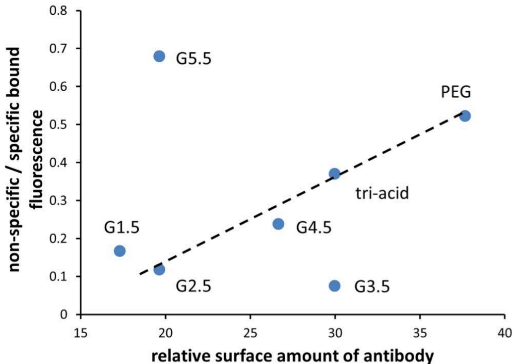
FIGURE 2. (A) (LH scale) Relative fluorescence signal for the covalently-bound antibody, binding of its specific antigen and of a non-specific antigen for a range of surface linkers. (RH scale) Surface density of antibody, determined by neutron reflection. PMMA here refers to the oxidised surface. (B) Fluorescence signal for both specifically and non-specifically bound antigen against the relative amount of surface bound antibody determined by fluorescence. (C) Fluorescence signal ratio of non-specific / specific antigen against the relative amount of surface bound antibody determined by fluorescence. Specific and non-specific antigen concentration for fluorescence measurement: 5 \mu\text{g/mL}
