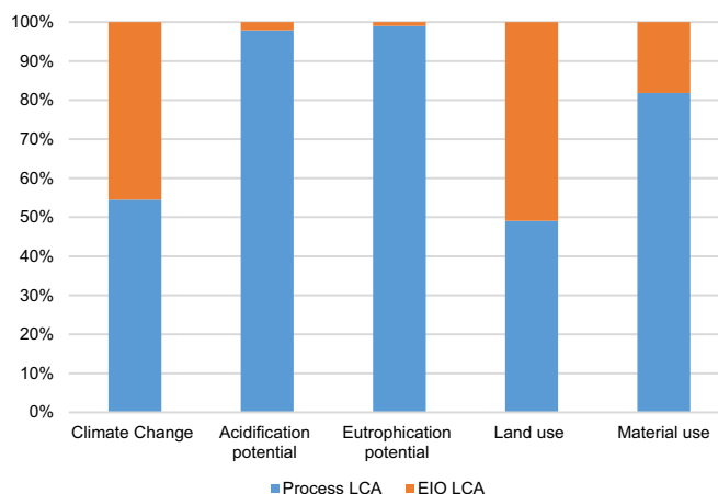
Fig. 10. Results of hybrid LCA of Module A across key sustainability metrics.
