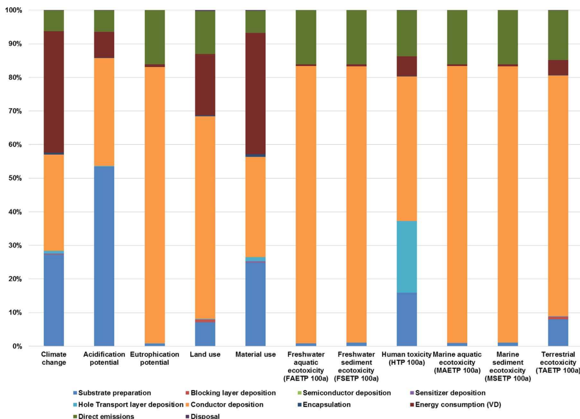
Fig. 11. Environmental profile of all the unit process exchanges in 1 m² PSC based on process-based data.
