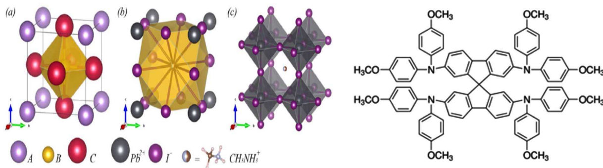
Fig. 2. Perovskite ABX_3 structure (left) and SPIRO-OMeTAD molecule (right). Adapted from Ref. [75] with permission of the Copyright© 2015, American Chemical Society.
