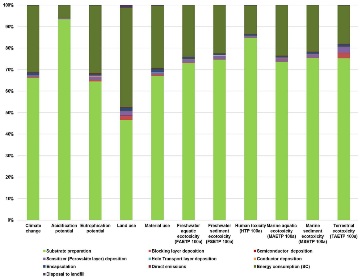
Fig. 14. Environmental profile of all the unit process exchanges in 1 m² PSC Module B.
