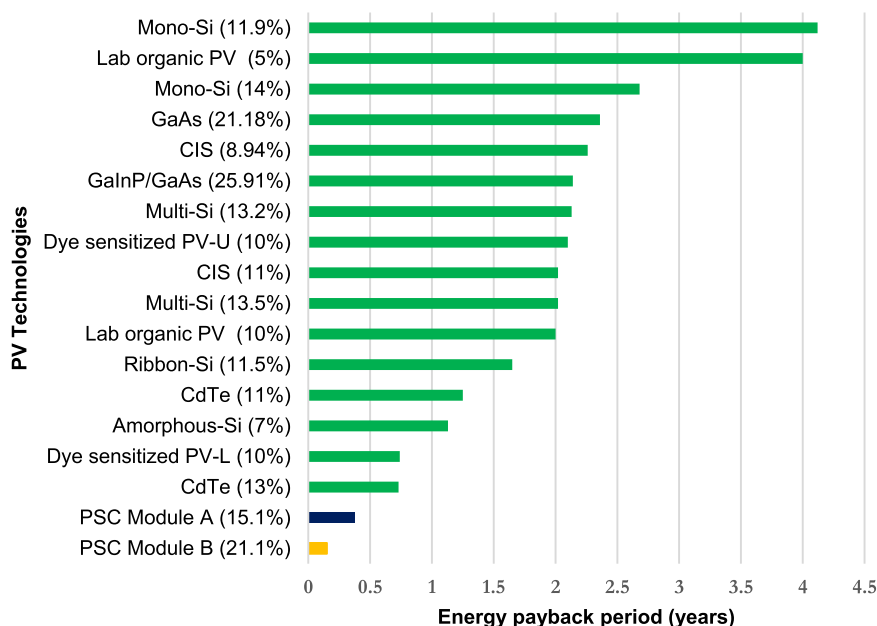
Fig. 16. Comparison of EPBP of existing PV technologies with PSC. Data for other PV technologies are obtained from Garcia-Valverde et al. [10].
