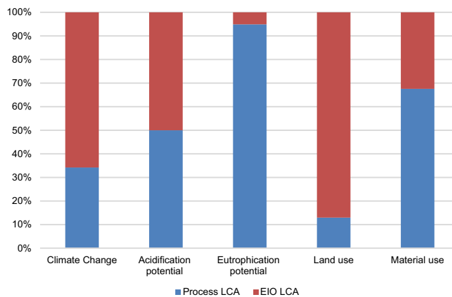
Fig. 13. Results of hybrid LCA of Module B across key sustainability metrics.
