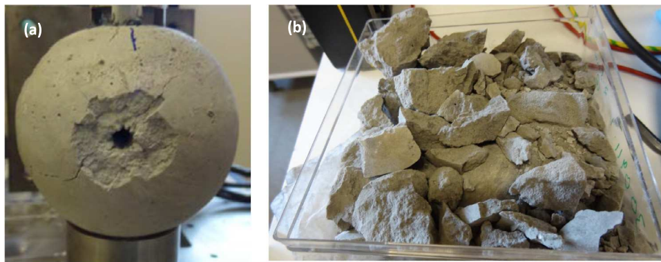
Fig. 4. Targets after impact. (a) Cratering event. (b) Catastrophically disrupted target.
