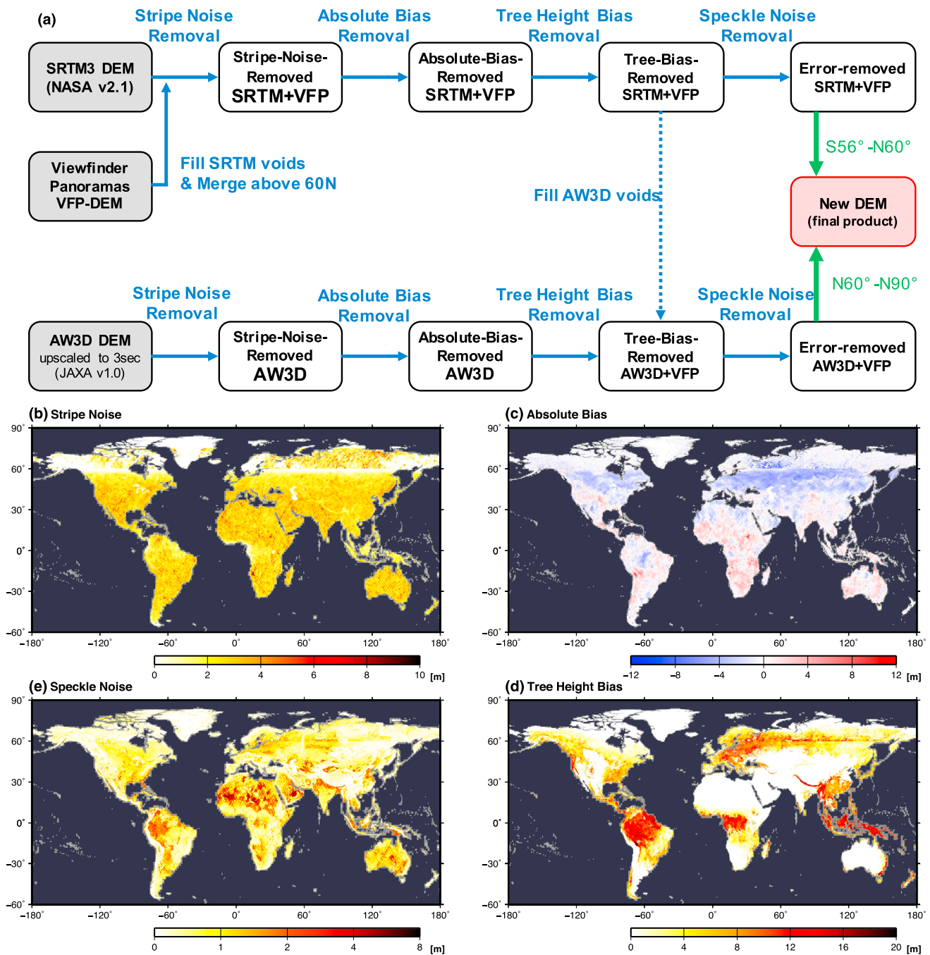
Figure 1. Procedures of error removal. Schematic diagram. Spatial pattern of detected errors of error removal procedures. The 90th percentile value in each 0.1° tile is shown for (b) stripe noise, (c) absolute bias, (d) tree height bias, and (e) speckle noise. The absolute magnitudes are shown for stripe and speckle noise for clear visualization purpose. The discontinuity around N60° corresponds to the boundary of the SRTM and AW3D DEMs.
