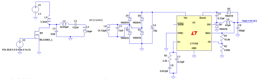
Figure 3. CoilMove transmit circuit on the left and receive circuit on the right, separated by two inductors.
