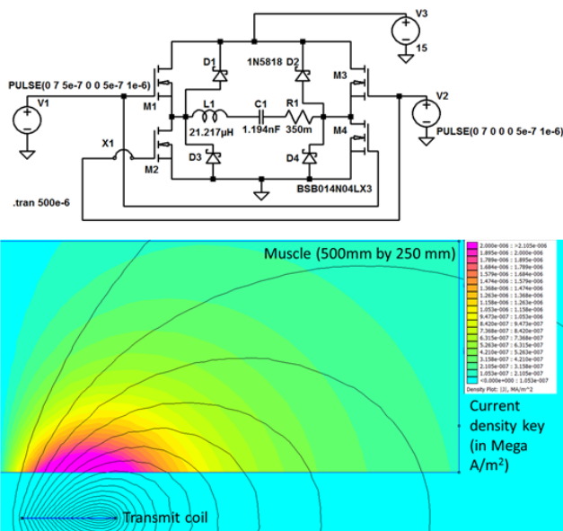
Figure 2. Upper: an LTSpice simulation of the MagneticMIMO and MultiSpot systems. Lower: A FEMM simulation to estimate the current density induced in a user's muscle tissue by the MagneticMIMO and MultiSpot systems.
