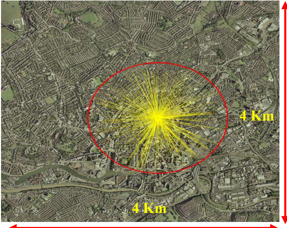
Figure 3. An exemplary LTE-800MHz macro-cell scenario.
