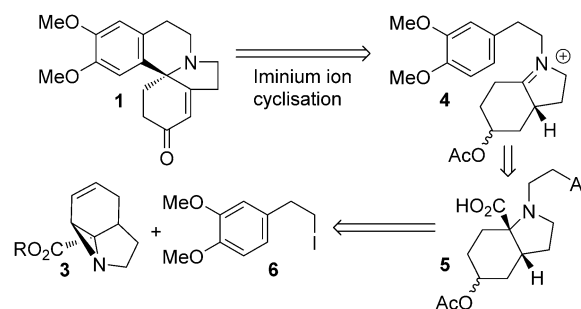
Scheme 1. Synthesis and reactivity of tricyclic aziridines and initial retrosynthetic analysis of 3-demethoxyerythratidinone ( 1 ).
