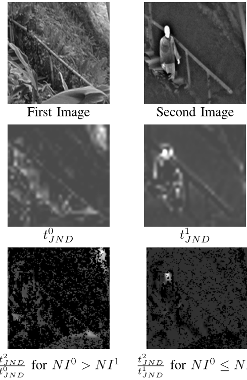
Fig. 5. Example visualisation of intermediate fusion measures. First row: Original images. Second row: JND thresholds t_{JND}^l . Bottom row: Correction factors t_{JND}^2/t_{JND}^l .
