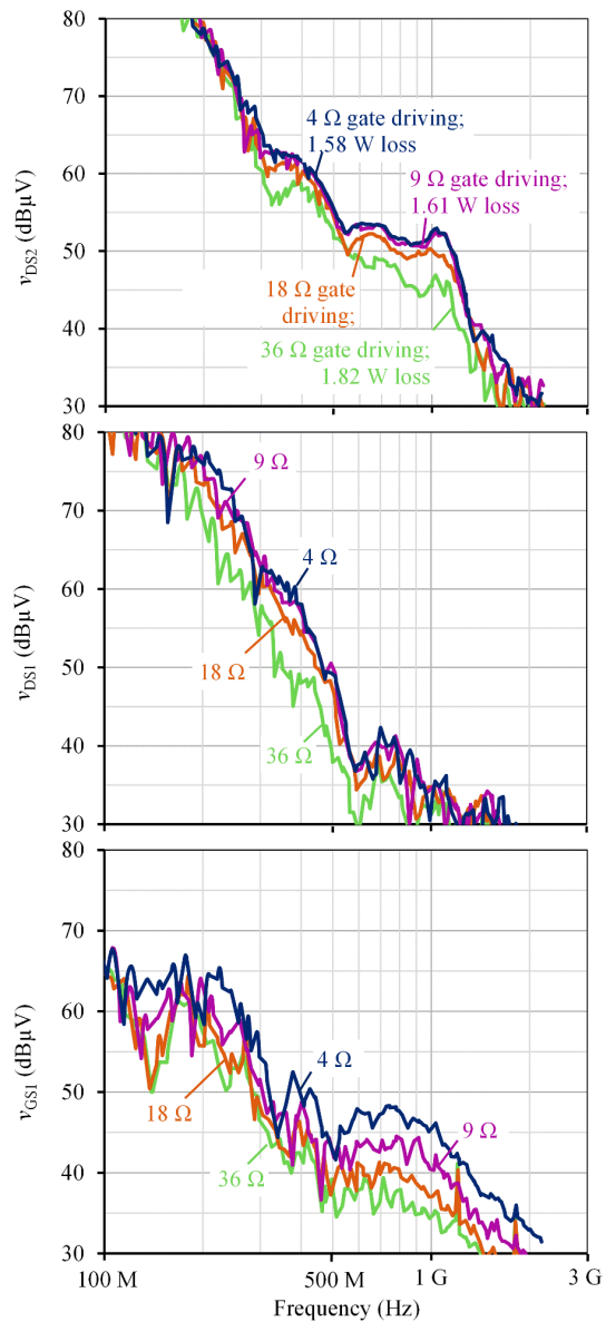
Fig. 20. Spectral envelopes, calculated from the measured time-domain data of complete switching cycles, for the four gate-driving scenarios in Fig. 22.
