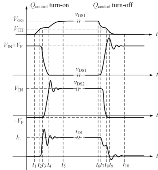
Fig. 7. Representative switching waveforms of v_{GS1} , v_{DS1} , v_{DS2} , and i_{D1} , and the delineation of 8 control phases.
