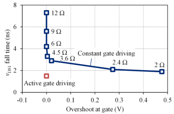
Fig. 16. Measured v_{DS1} 97%-3% fall time vs. gate overshoot for the control GaN FET under constant-strength and active gate-driving scenarios.
