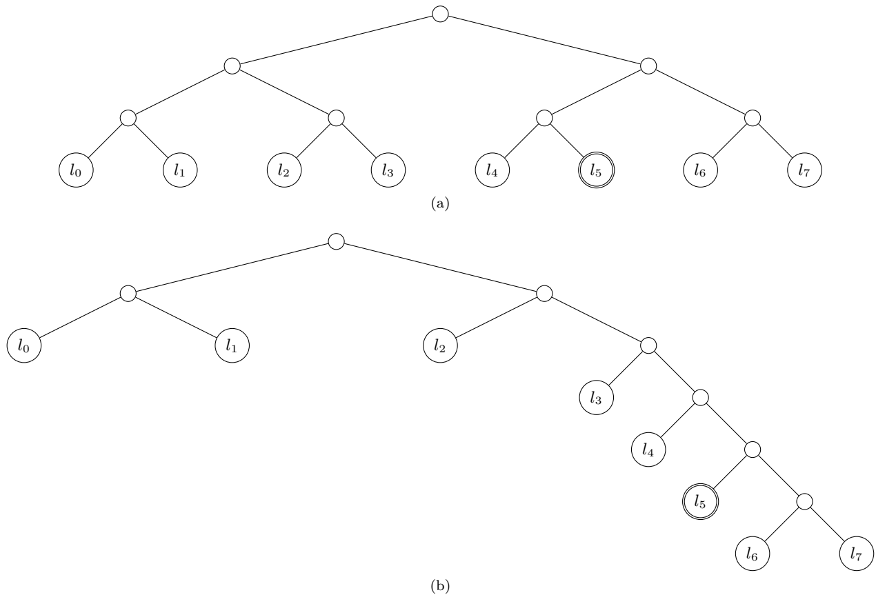
FIG. 1. Example backtracking trees, where l_5 is a leaf corresponding to a solution to a constraint satisfaction problem: (a) shows an example of a perfectly balanced backtracking tree, where each leaf can be associated with a 3-bit string corresponding to a path to that leaf; (b) on the other hand shows an example of an unbalanced backtracking tree, where specifying a path to a leaf requires 6 bits.
