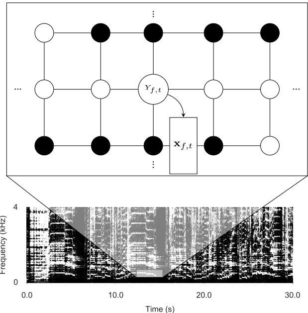
Fig. 1. Conditional Random Fields for singing voice separation. Feature vector \mathbf{x}_{f,t} is computed for each pixel in a spectrogram. This alone can be used to classify Y_{f,t} as either vocal (shown here in white) or non-vocal (black). However, we may also make use of the neighbours of Y_{f,t} to assist with prediction.
