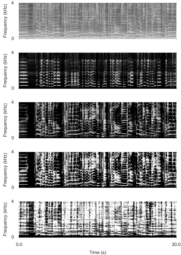
Fig. 2. Example output from our system. From top to bottom: log power spectrogram of mixture, Deep Learning system, REPET system, our proposed method (4-connected model), Ideal Binary Mask. In all images white indicates high energy.
