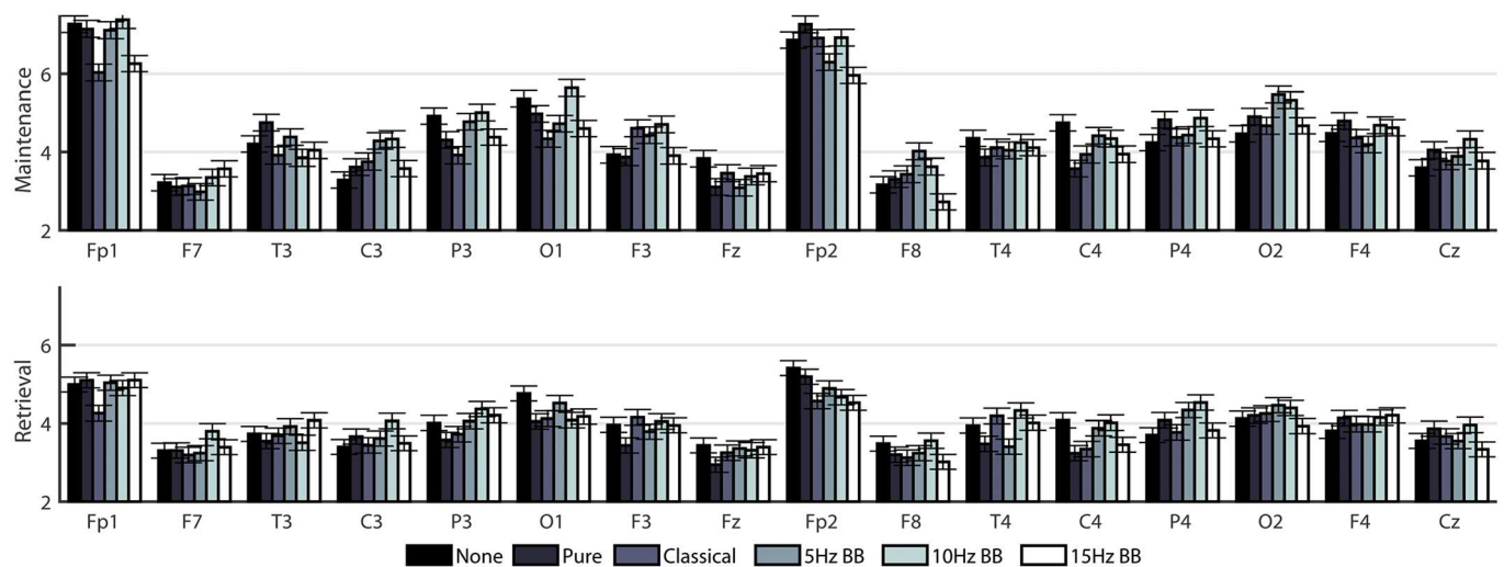
Fig 8. Mean betweenness centrality of EEG nodes in cortical networks for all six acoustic stimulation conditions. Bars indicate standard error.
