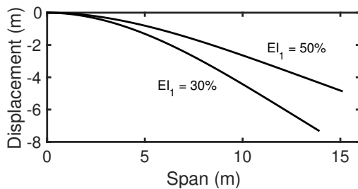
Figure 13: Spanwise wing deformation at low airspeed ( V = 8 \text{ m/s} ) for out-of-plane stiffness above and below threshold.
