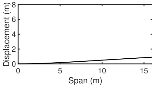
Figure 5: Spanwise wing deformation at airspeed before flutter ( V = 22 \text{ m/s} ).
