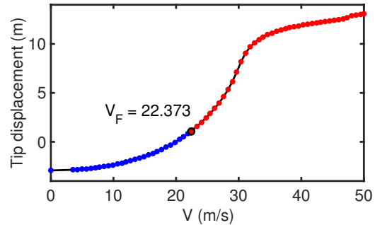
Figure 3: Variation of steady state tip displacement with airspeed (linear C_L ). Hopf bifurcation ( V_F ) occurs at 22.373 m/s. Blue and red curves indicate stable and unstable equilibria respectively.
