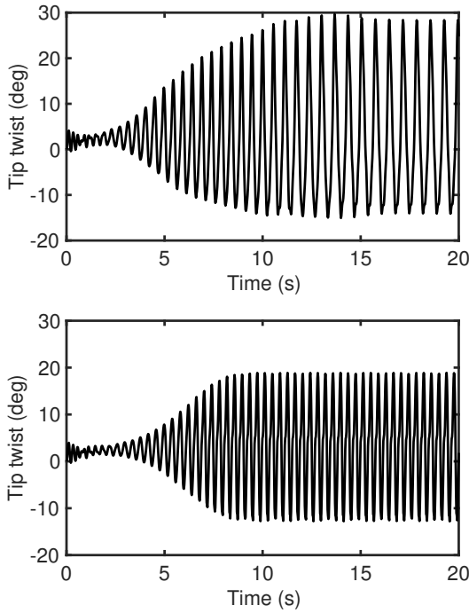
Figure 9: Time histories for V = 25 \text{ m/s} (linear C_L and nonlinear C_L respectively).
