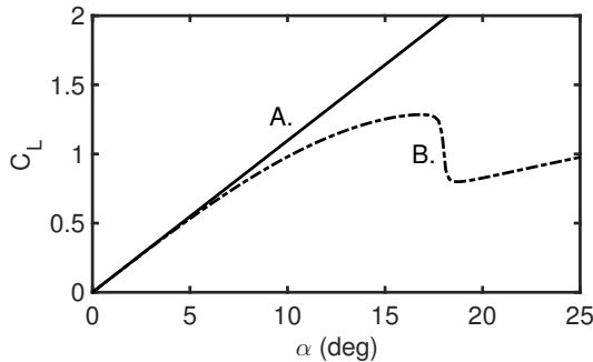
Figure 2: C_L functions for linear (non-stall) and nonlinear (stall) cases. The nonlinear curve is fully stalled at \alpha \approx 17^\circ .
