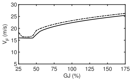
Figure 12: Variation of flutter velocity with torsional stiffness (solid = linear C_L , dashed = nonlinear C_L ).
