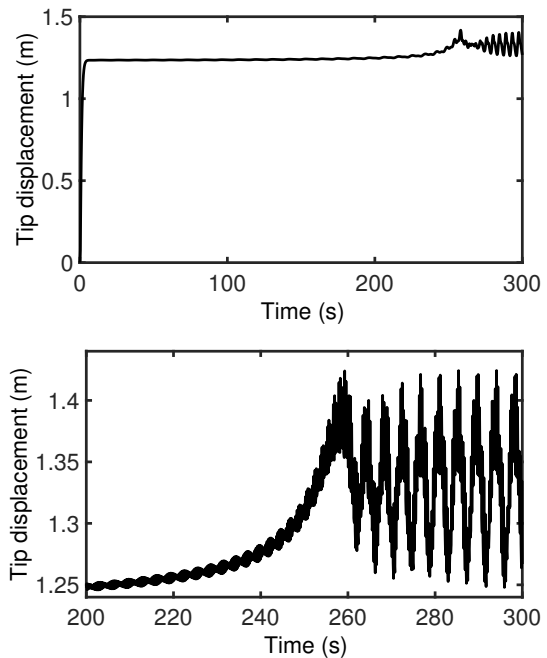
Figure 17: Time history for V = 23.24 m/s (nonlinear C_L ), showing LCO observable below the flutter velocity. This indicates the occurrence of a subcritical Hopf bifurcation. Note: the lower plot is a magnification of the upper plot.
