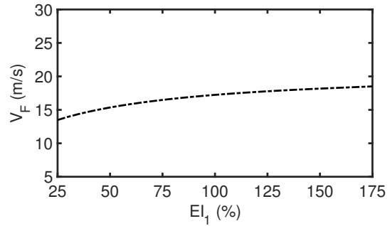
Figure 14: Variation of V_F with EI_1 with gravitational effect excluded (linear C_L = solid, nonlinear C_L = dashed).
