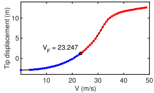
Figure 6: Variation of steady state tip displacement with airspeed (nonlinear C_L ). Hopf bifurcation ( V_F ) occurs at 23.247 \text{ m/s} .
