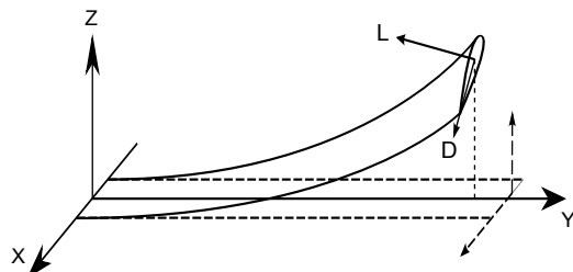
Figure 1: High aspect ratio wing deformation showing re-orientation of aerodynamic forces and effective tip shortening.
