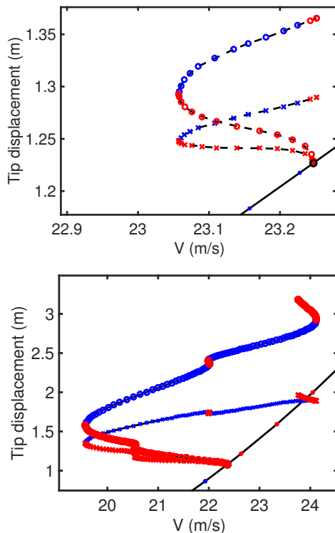
Figure 18: Variation of steady state tip displacement with airspeed (nonlinear and linear C_L ; upper and lower respectively), showing maxima (circle) and minima (cross) of periodic solution emanating from Hopf bifurcation. Presence of solution below V_F is indicative of subcritical behaviour in both cases.
