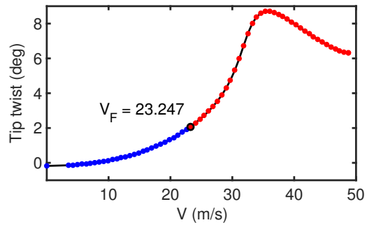
Figure 7: Variation of steady state tip twist with airspeed (nonlinear C_L ). Hopf bifurcation ( V_F ) occurs at 23.247 \text{ m/s} .
