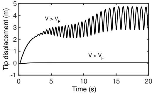
Figure 4: Time histories for V = 20 \text{ m/s} and V = 25 \text{ m/s} (linear C_L ), demonstrating behaviour before and after Hopf bifurcation.
