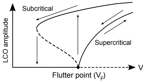
Figure 16: Diagram showing LCO amplitude vs. velocity for the two generic Hopf bifurcations. Subcritical case shows LCO below V_F . Supercritical case is reversible whereas subcritical case exhibits hysteresis loop.
