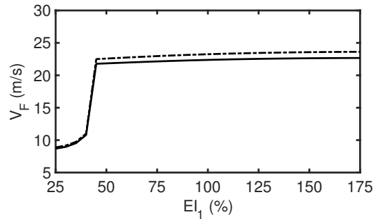
Figure 10: Variation of flutter velocity with out-of-plane bending stiffness (solid = linear C_L , dashed = nonlinear C_L ).
