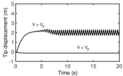
Figure 8: Time histories for V = 20 \text{ m/s} and V = 25 \text{ m/s} (nonlinear C_L ), demonstrating behaviour before and after Hopf bifurcation.
