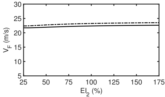
Figure 11: Variation of flutter velocity with in-plane bending stiffness (solid = linear C_L , dashed = nonlinear C_L ).
