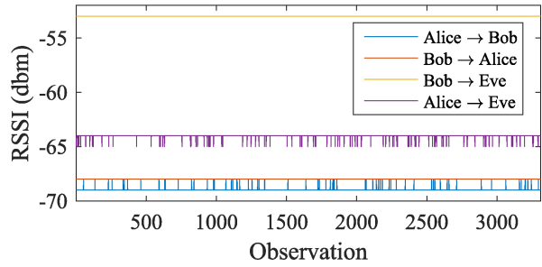
Fig. 3. RSSI of packets exchanged in the anechoic chamber.
