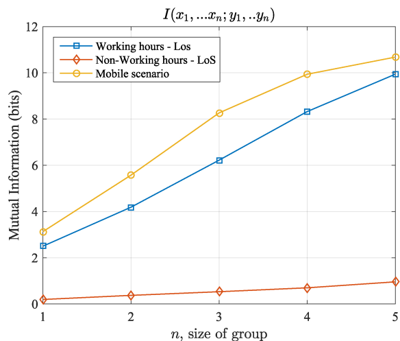
Fig. 7. Effects of using sequences of different sizes of RSSI values as x_i .
