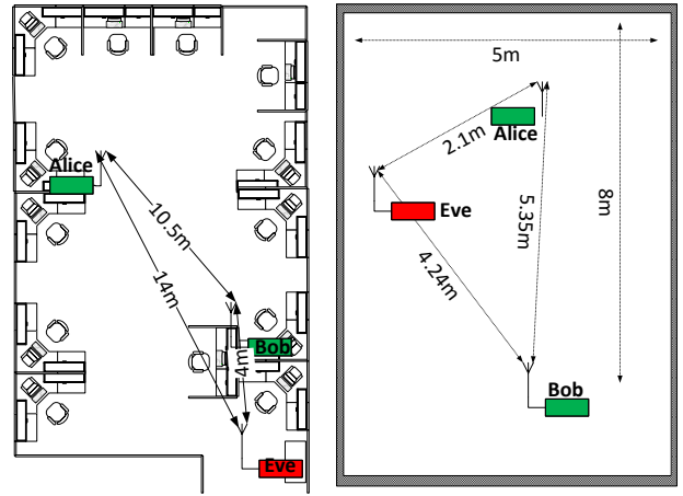
Fig. 2. Left: Layout of experiment in office space. Right: Layout of experiment in the anechoic chamber.
