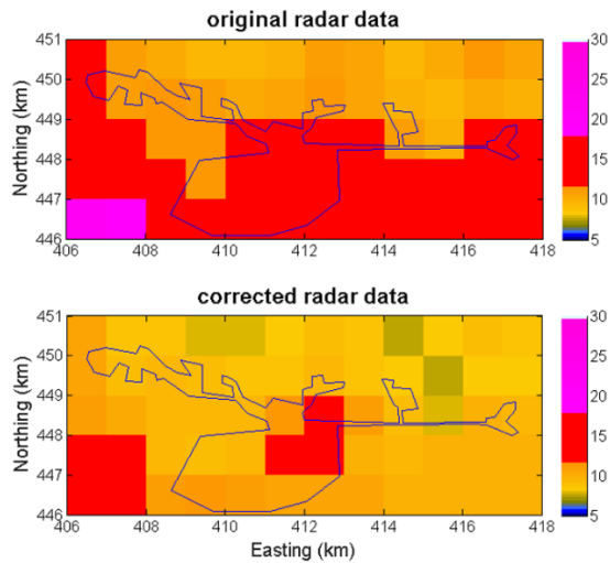
Figure 8. Original 5 min radar data (top) and corrected 5 min radar data (bottom) on 9 th January 2008 at 21:20:00
