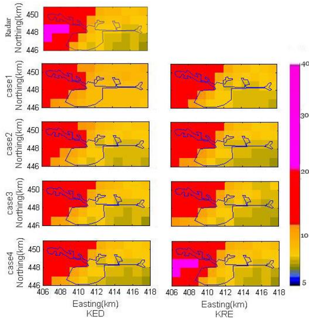
Figure 7. Merged rainfall on 6 th of September 2008 for the KED merging method (left) and KRE method (right) and for the four cases of merging network. The top plot is the original radar data.
