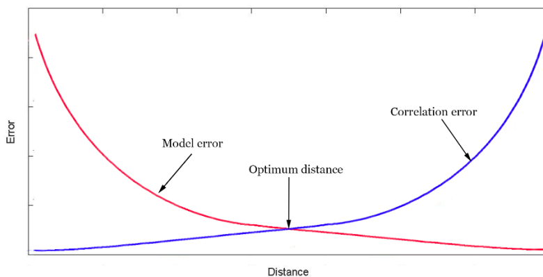
Figure 5. Schematic plot showing the optimum distance of merging network away from the study area.
