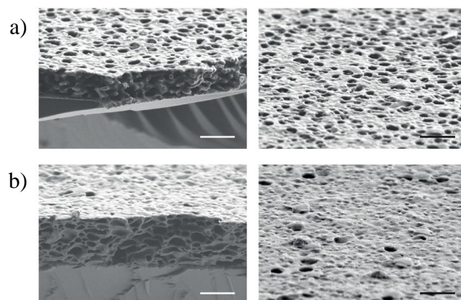
Figure 12. Cross-sectional and surface SEM images of PFS-VImTf 2 N/PAA porous membranes after oxidation at 0.6 V for 10 min (a), and then reduction at -0.2 V for 10 min (b). Scale bars are 1 μm. Reproduced with permission from reference 146.
