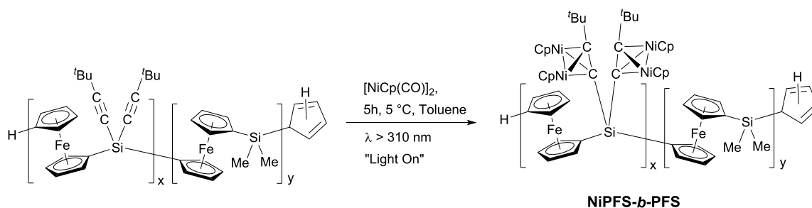
Scheme 19. Synthesis of highly metallised NiPFS- b -PFS through post-polymerisation functionalisation of acetylidePFS- b -PFDMS with [NiCp(CO)_2] .
