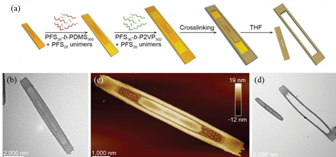
Figure 48. (a) Schematic representation for the formation of uniform concentric and hollow rectangular platelet micelles; (b) TEM and (c) AFM images of a concentric rectangular micelle and (d) TEM image of a perforated rectangular platelet micelle and the corresponding rectangular ring platelet micelle after crosslinking and subsequent dissolution of the non-crosslinked segment. Reproduced with permission from reference 385 .
