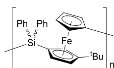
Figure 8. Poly(ferrocenyldiphenylsilane) with a tert -butyl substituent per ferrocenediyl.
