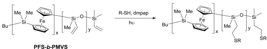
Scheme 20. Functionalisation of polyferrocenyldimethylsilane- block -polymethylvinylsiloxane ( PFMS- b -PMVS ) via a UV initiated thiol-ene “click” reaction.
