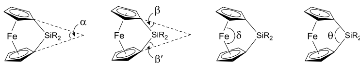
Figure 2. Geometric parameters used to describe the structure of [1]ferrocenophanes.
