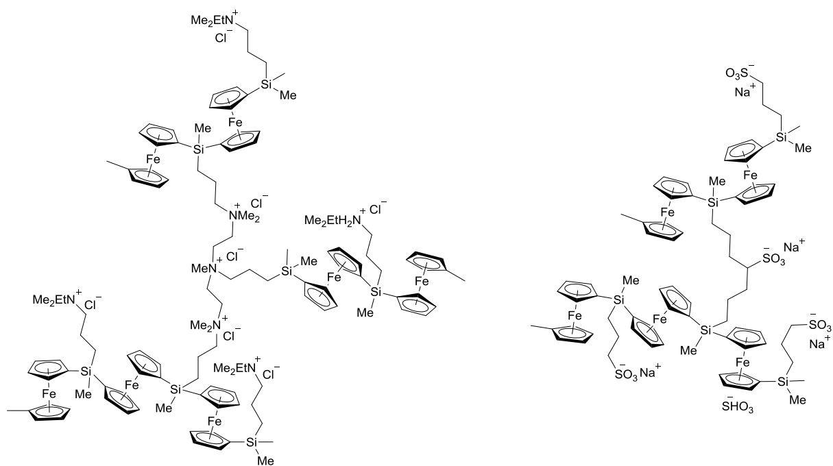
Figure 11. Permanently charged cationic and anionic PFS networks.
