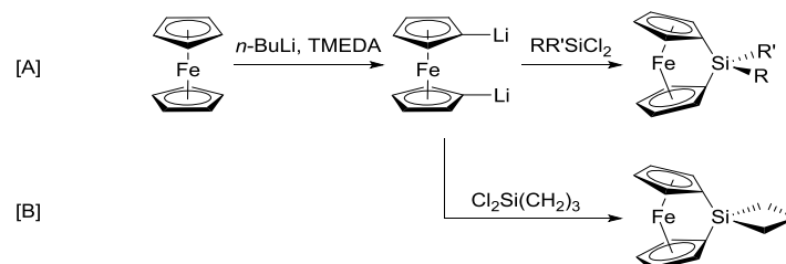
Scheme 2. Synthesis of sila[1]ferrocenophanes from ferrocene.
