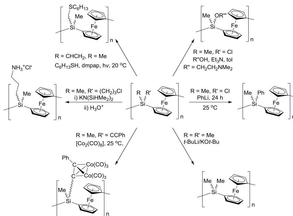
Scheme 8. Examples of post-polymerisation functionalisation methods for polyferrocenylsilanes.
