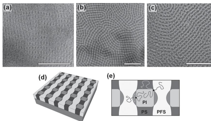
Figure 34. TEM images of \mu -ISF (a) before staining and (b) after staining with OsO 4 ; (c) SEM image of bottom interface of \mu -ISF; schematics showing (d) thin film patten and (e) its chain conformation within the microdomain. Scale bars are 300 nm. Reproduced with permission from reference 315.
