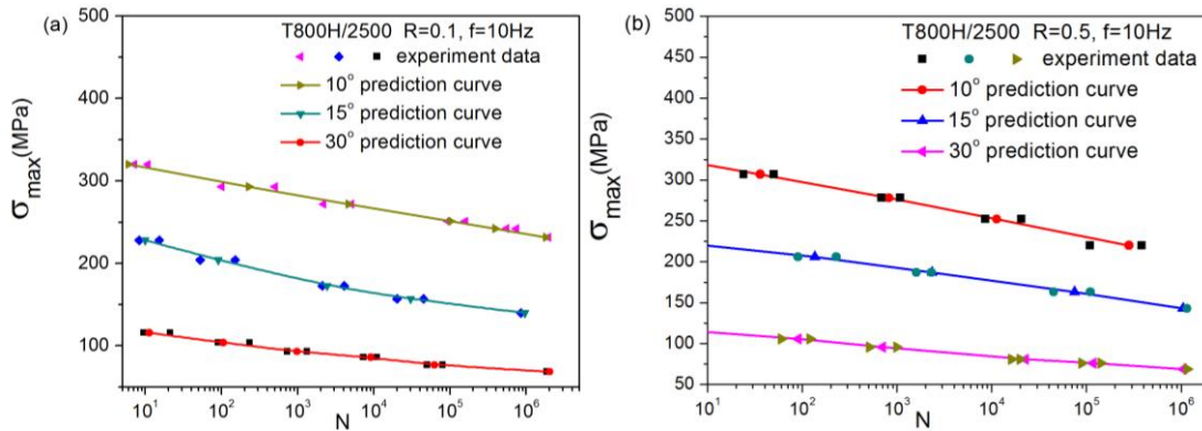
Fig. 6. 10°, 15° and 30° CFRP lamina predicting S-N relationships under (a) R=0.1 and (b) R=0.5
