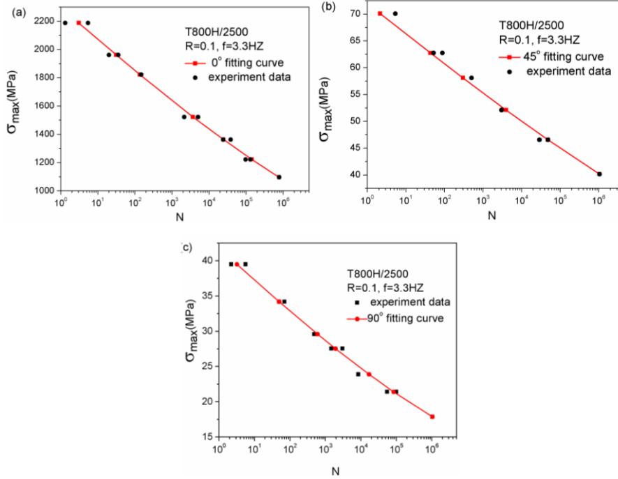
Fig. 3. Fitting S-N relationships for CFRP composite lamina under R=0 (a) 0^\circ (b) 45^\circ (c) 90^\circ
