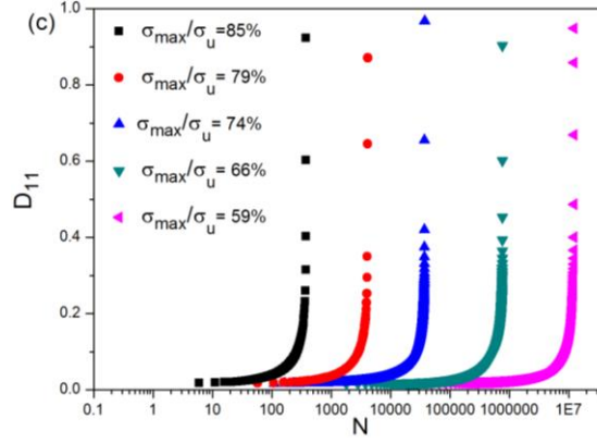
Fig. 9. Fatigue damage growths on meso-scale for GFRP 19° unidirectional composite laminate under R=0.5 : (a) transverse damage D_{22} , (b) shear damage D_{12} , (c) axial damage D_{11}
