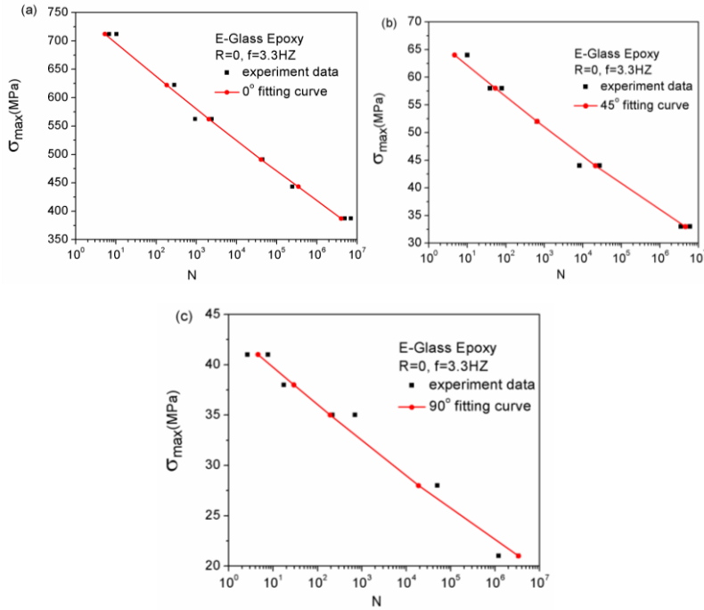
Fig. 2. Fitting S-N relationships for GFRP composite lamina under R=0 : (a) 0^\circ , (b) 45^\circ (c) 90^\circ
