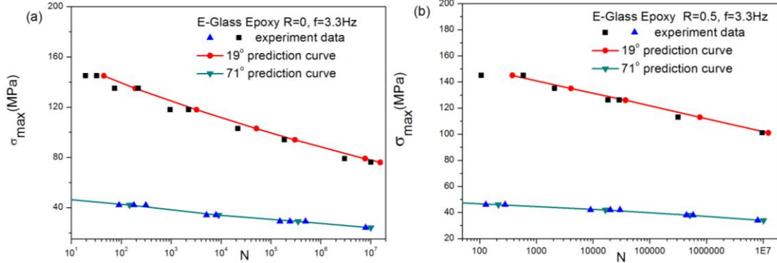
Fig. 5. 19° and 71° GFRP unidirectional laminate predicting S-N relationships (a) under R=0 (b) under R=0.5
