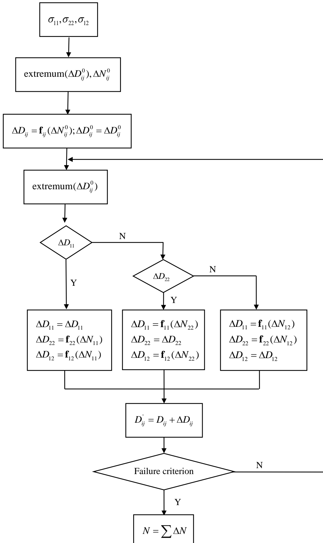
Fig. 4 Flow chart of the present numerical simulation
