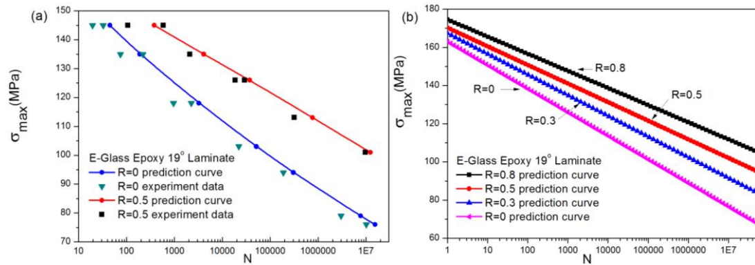
Fig. 7. Off-axis fatigue behavior for the E-Glass Epoxy 19^\circ unidirectional composites: (a) comparison of the fatigue life between R=0 and R=0.5 (b) prediction S-N curves group at R=0, 0.3, 0.5, 0.8
