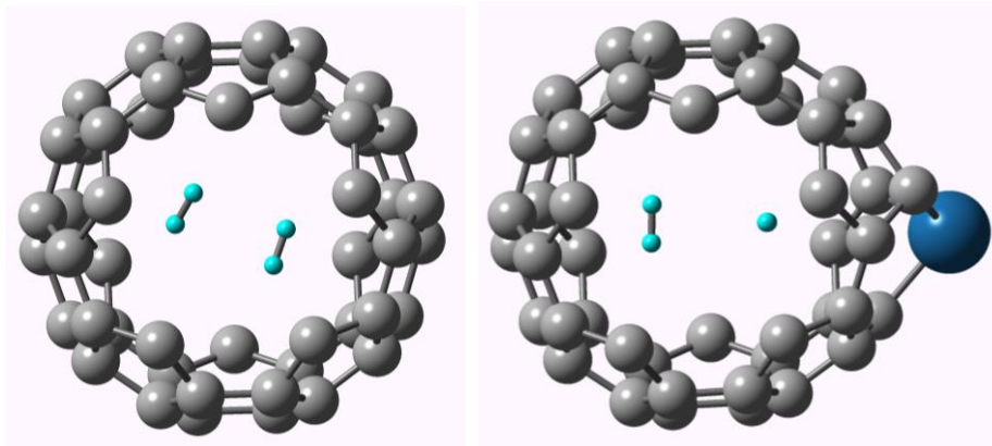
Figure 9 – Undoped C 60 fullerene (left) and C 60 with substitational Pt (right) optimized with two internal H 2 molecules showing the change in orientation of the H 2 molecules caused by the presence of a substitational Pt dopant. The bottom and topmost five carbon atoms have been excluded to observe the H 2 molecules more clearly, calculated with B3LYP and LANL2MB (C = grey, H = light blue, Pt = dark blue).
