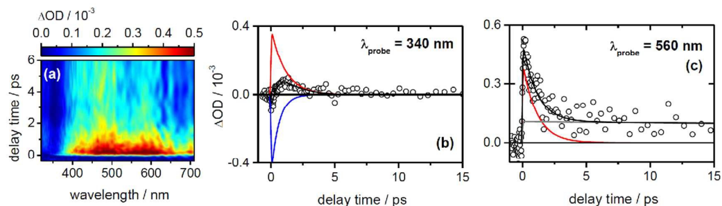
Fig. 3. (a) Two-dimensional false colour intensity map of the TEA spectrum obtained from C ( c_0 = 10 mM) in \text{CHCl}_3 following excitation at 260 nm ( C = 65\% , C \cdot C = 35\% ). Absorption change profiles as a function of delay time obtained from (a) at probe wavelengths of (b) \lambda_{\text{probe}} = 340 nm and (c) \lambda_{\text{probe}} = 560 nm. Open circles = experimental data, black line = total fit. Coloured lines are decay components with time constants of \tau_1 = 0.6 ps (blue line), \tau_2 = 1.1 ps (red line) and \tau_3 = 193 ps (grey line). See Table 2 for details of \tau_n fit amplitudes ( A_n ).
