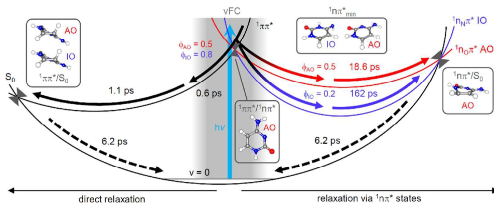
Fig. 5. Schematic potential energy cuts through the S_0 , ^1\pi\pi^* , ^1n_0\pi^* and ^1n_N\pi^* electronic states for the AO and IO tautomers of dC, depicting a plausible kinetic scheme for the excited state relaxation of dC in chloroform based on TVAS and TEAS measurements with 260 nm excitation. Black = IO and AO, Red = AO only, Blue = IO only. Possible structures involved in the relaxation dynamics are obtained from theoretical calculations on the AO and IO tautomers of the simpler cytosine nucleobase in the gas-phase; ^1\pi\pi^*/S_0 AO and ^1\pi\pi^*/^1n\pi^* AO from Ref. 37, ^1n\pi^*/S_0 AO and ^1n\pi^*_{\min} AO from Ref. 38, ^1\pi\pi^*/S_0 IO and ^1n\pi^*_{\min} IO from Ref. 27. The values of \phi denote branching between competing channels.
