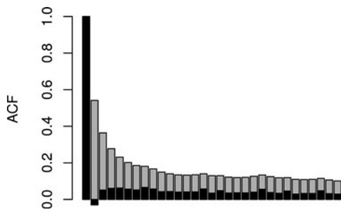
Figure 3. Aggregate ACF for model (1) residuals assuming independent residuals in gray, with the equivalent for the standardized residuals assuming AR1 residuals, overlaid in black. While not perfect, the AR1 model greatly reduces the unmodeled temporal autocorrelation.
