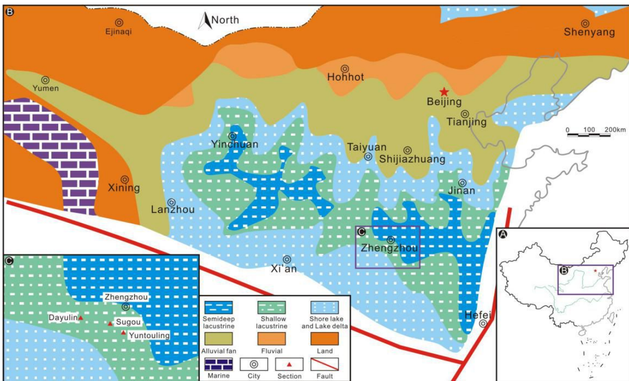
Figure S2. Latest Permian paleogeographic map of North China (modified from Zhu, R.K., Deng, S.H., Xu, H.X., and Guo, H.L., 2007, Lithofacies palaeogeography of the Permian in northern China: Journal of Palaeogeography 9, 133-142. Figure 3). A: Territory of China; B: Lithofacies paleogeography of the Latest Permian in Northern China; C: The red triangles show the location of studied sections: Dayulin, Sugou and Yuntouling sections. D.L.C. modified this figure after Zhu et al. (2007) using CorelDRAW14.
