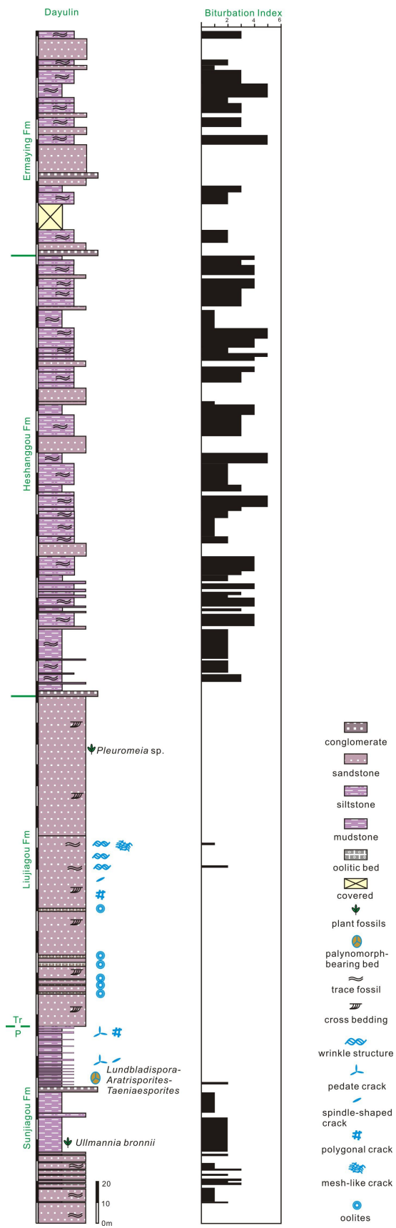
Figure S4. Bioturbation index of Dayulin section. D.L.C. created this figure using CorelDRAW14.
