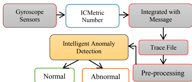
Fig. 1: ICMetric-IDS Architecture
