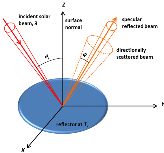
Figure 1. Scheme of the solar specular reflectance.
