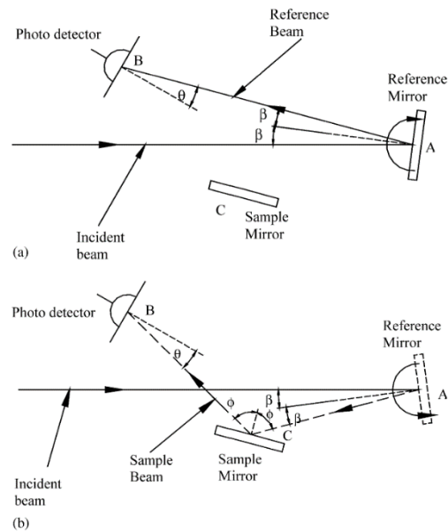
Figure 32. Basic principle of the new reflectometer by Malaysia University. (a): Measurement of the reference signal; (b): measurement of the sample signal [91].
