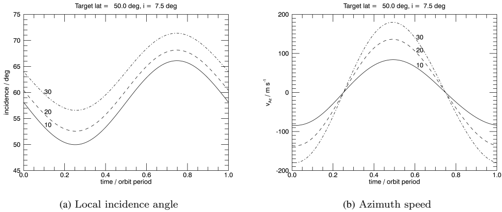
Figure 3 Azimuth speed and local incidence angle during the whole orbit period for points at latitude 50^\circ , and longitude offsets from the satellite of 10 , 20 and 30^\circ .
