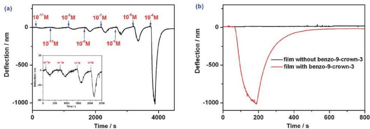
Figure 13. (a) Bending response for hydrogel layer coated in silicon microcantilever on the passage of various concentration of \text{Be}^{2+} from 10^{-11}\text{ M} to 10^{-4}\text{ M} with 0.01\text{ M} Tris-HCl buffer solution (pH 7.04). The inset depicts the magnified curve, (b) Bending response for hydrogel layer coated in silicon microcantilever with and without benzo-9-crown-3 [54]. Reprinted with permission. [54]. Copyright 2012 Royal Society of Chemistry.
