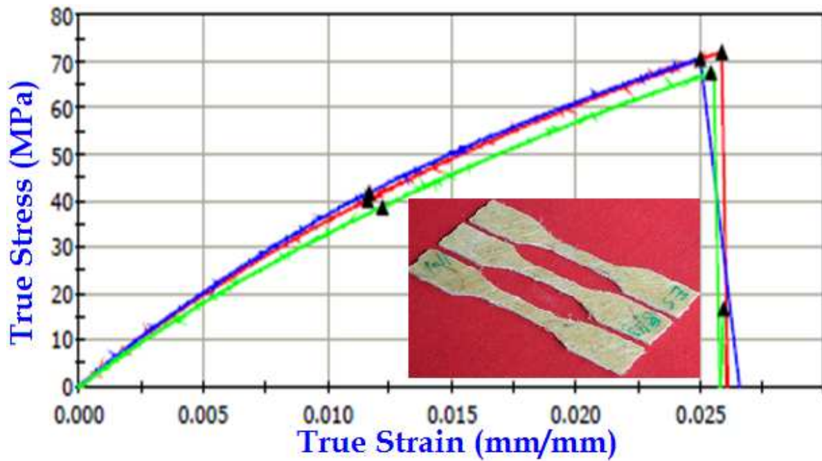
Fig. 5 (a) Tensile stress strain curve of sisal fibers perform mat reinforced composites and photographic image of tensile test cut specimens of sisal fibers perform mat reinforced composites (inset).
