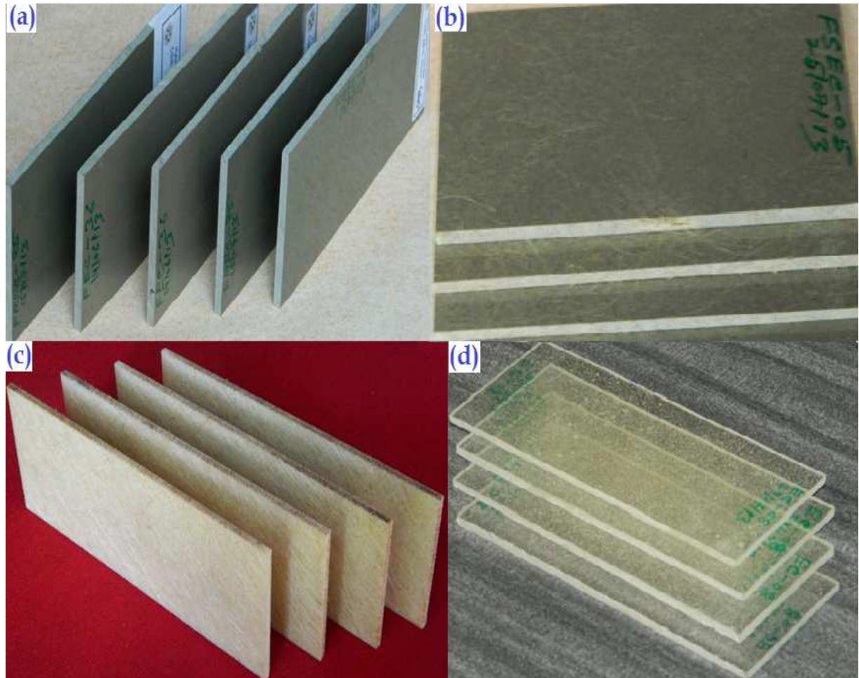
Fig. 2 Photographic images of (a) Fly ash fortified epoxy composite (FEC) (b) Hybrid green composites made out of fly ash and sisal fibres (HBC) (c) Sisal chopped fibers perform mat reinforced epoxy composites (SEC) (d) Neat epoxy (NE)
