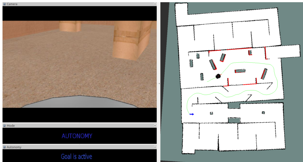
Figure 4.1: The control interface as presented to the operator. Left: video feed from the camera, the control mode in use and the status of the robot. Right: The map showing the position of the robot, the current goal (blue arrow), the AI planned path (green line), the obstacles' laser reflections (red) and the walls (black).
