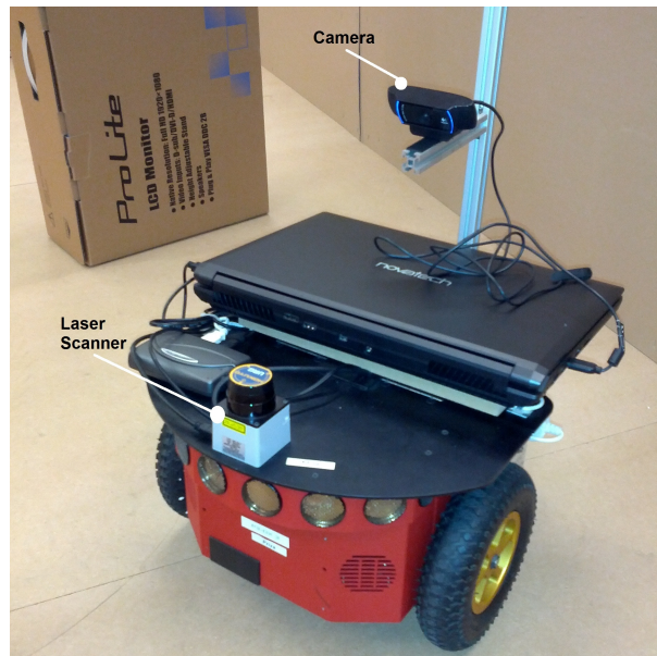
Figure 3.1: The pioneer-3DX robot used in the experiment, equipped with a laser range finder and a camera.
