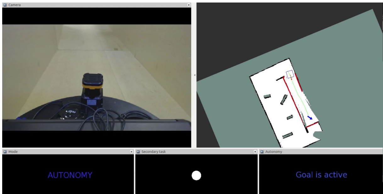
Figure 3.2: The control interface as presented to the operator. Top : video feed from the camera and the map of the environment. Inside the map, the position of the robot is visualized by the 3D model, the current goal by the blue arrow, the AI planned path by the green line, the obstacles' laser reflections by red and map walls with black. Bottom : the current autonomy mode, secondary task, and the status of the robot.
