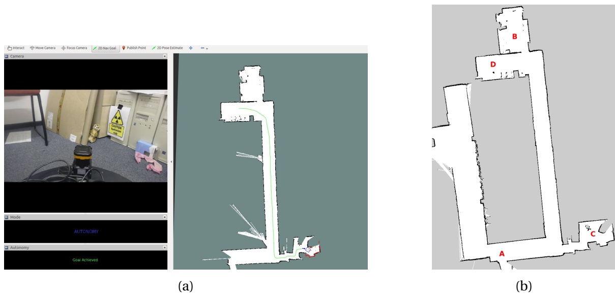
Figure 5.11: 5.11a: The control interface as presented to the operator. Left: video feed from the camera, the control mode in use and the status of the navigation goal. Right: The map showing the position of the robot (blue footprint and red arrow), the current goal (blue arrow), the AI planned path (green line), the obstacles' laser reflections (red) and the walls (black). 5.11b: The SLAM map of the arena as displayed to the human operator on the interface. Operators had to navigate in turn from point A; to B; to C; to D; and then back again to point A.
