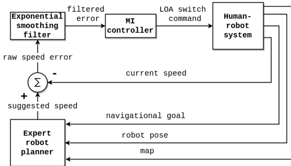
Figure 5.1: The block diagram of the MI control system. Given a navigation goal; the current pose of the robot; and the map (or a known surrounding area); the expert planner yields a close-to-optimal suggested speed. This speed denotes how fast the robot should be moving towards achieving the navigation goal. Then this speed is compared with the current speed of the robot towards that goal to calculate the raw performance error. The MI controller decides on switching LOA based on the filtered error.
