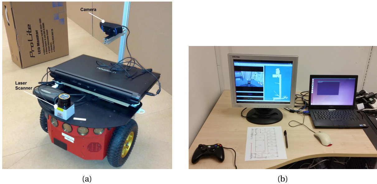
Figure 5.8: 5.8a: The pioneer 3DX robot used in the experiment. 5.8b: the Operator Control Unit (OCU), composed of a laptop, a joystick, a mouse and a screen showing the control interface. The same OCU was used in all variable autonomy experiments. Note the floor plan in front of the screen, used for the secondary task.
