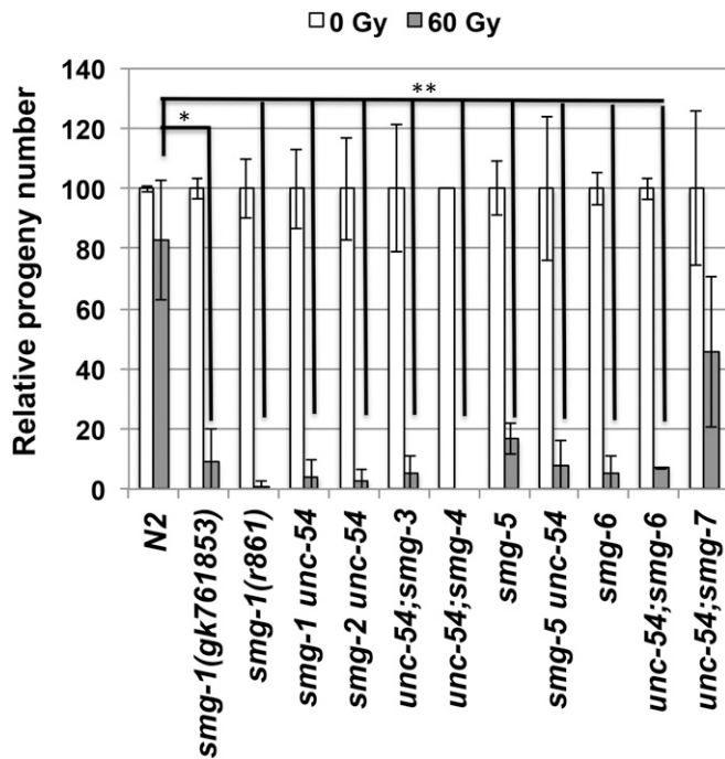
Figure 7 IR sensitivity of other NMD mutants: Early L1 larvae of N2, smg-1(gk761853) , smg-1(r861) , smg-1(r904) , unc-54(r293) , smg-2(r908) , unc-54(r293) , unc-54 (r293) ; smg-3 (r930) , unc-54 (r293) ; smg-4 (r1169) , smg-5 (r860) , smg-5 (r860) unc-54 (r293) , smg-6 (ok1794) , unc-54 (r293) ; smg-6 (r1217) and unc-54 (r293) ; smg-7 (r1197) were subjected to the indicated amounts of radiation, allowed to develop to young adult stage and lay eggs. After 12 hours worms were removed and eggs counted. The number of laid eggs normalized to that of the non-irradiated specimen for each strain is shown. Three plates with 3 worms each were scored for strain and condition. Error bars indicate SD. Asterisks indicate the level of significance as standard: * P = 0.01-0.05 , ** P = 0.001-0.01 , *** P < 0.001 .
