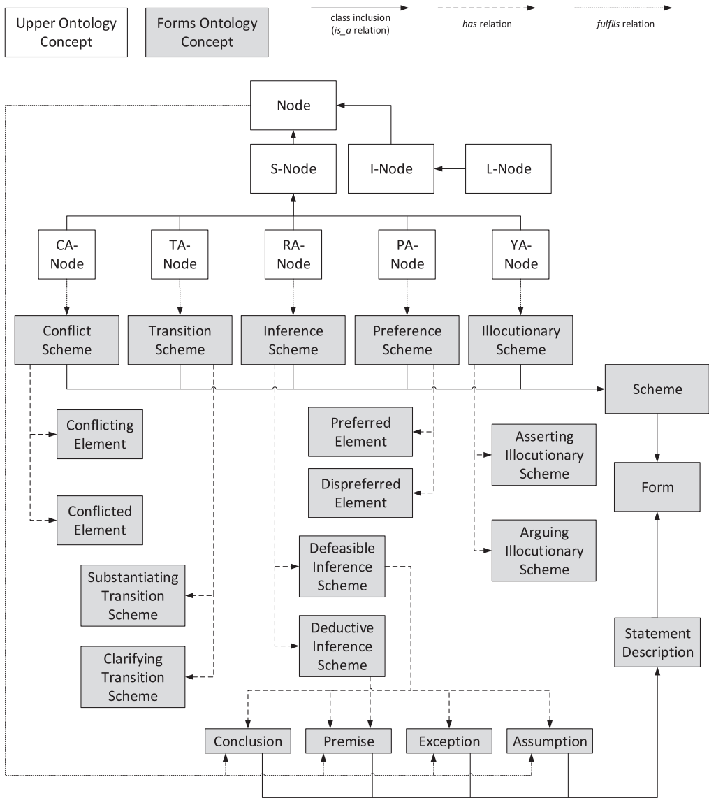
Fig. 1. AIF+ core ontology.
