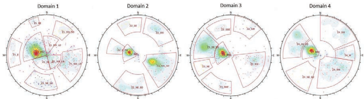
Fig. 2. Fracture Set Analysis for each Fracture Domain.
