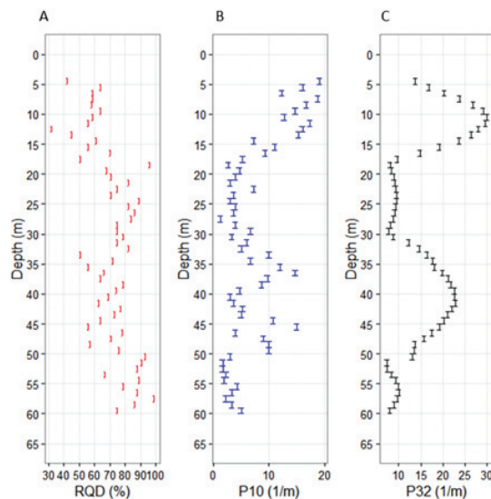
Fig. 3. (a) RQD, (b) P_{10} and (c) P_{32} determinations within the shaft.
