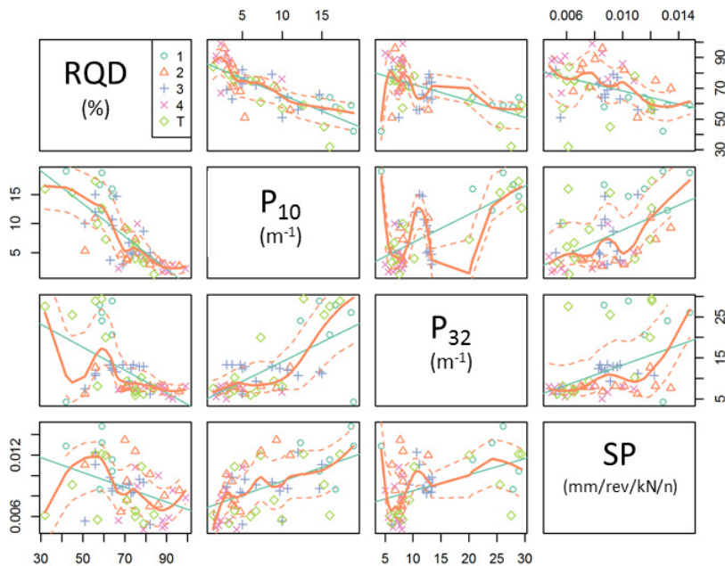
Fig. 4: Scatter matrix of different fracture measures against specific penetration rate for each fracture domain.
