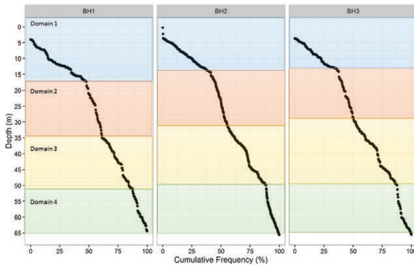
Fig. 1. Constant Fracture Intensity Domain (CFI) identified for each borehole. Domains are coloured for clarity.
