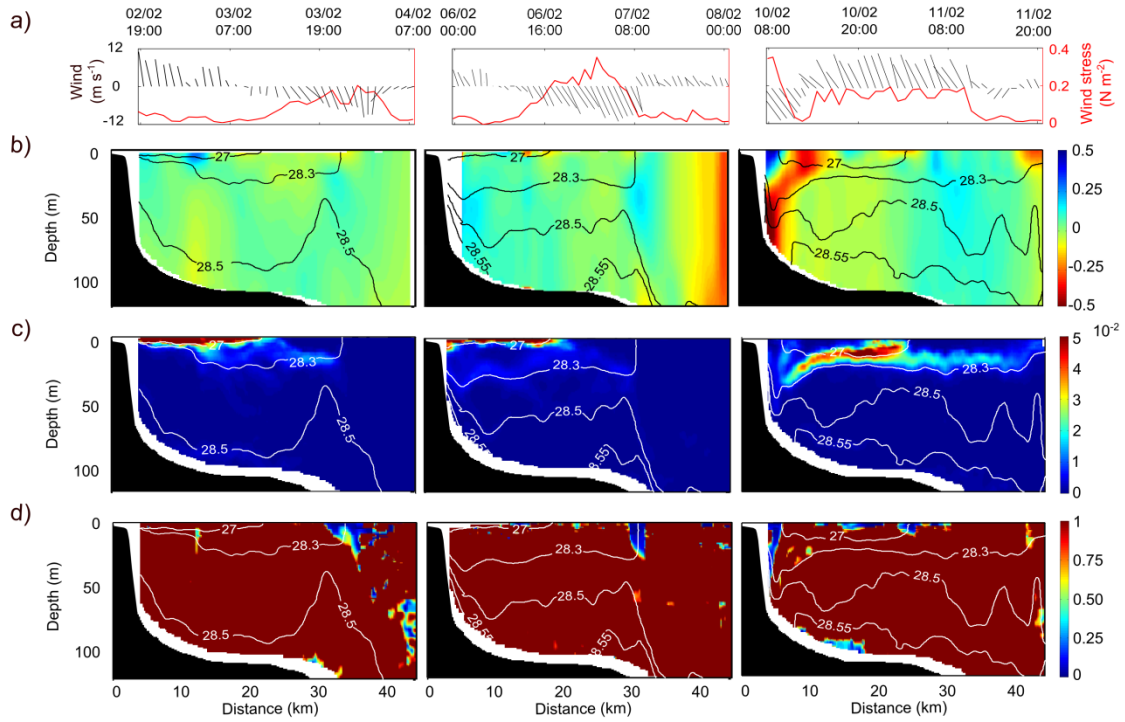
Figure 8 – a) Time-series of wind speed and direction (m s -1 ). The wind stress is shown in red (N m -2 ). Cross-shelf section of b) the along-shelf current (m s -1 ), c) the derived Brunt-Väisälä frequency (s -1 ) and d) the Richardson Number (dimensionless). Density contour lines are shown in black on the upper panel and in white on middle and lower panels.
