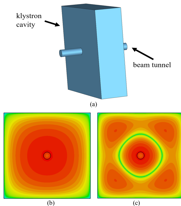
Fig. 1. The geometry of the cuboid cavity (a), and the electric field patterns of the TM_{110} (b) and TM_{330} modes (c).
