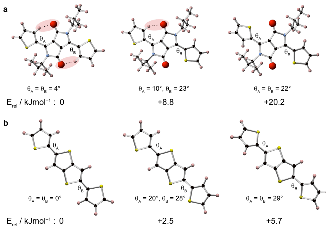
Figure 2. Comparison of optimized geometries and relative energies of DPP-thiophene units (top) and DTT units (bottom). Weak hydrogen bonds between the thiophene rings and the carbonyl groups in the DPP moiety, and torsion angles, \theta , are indicated.
