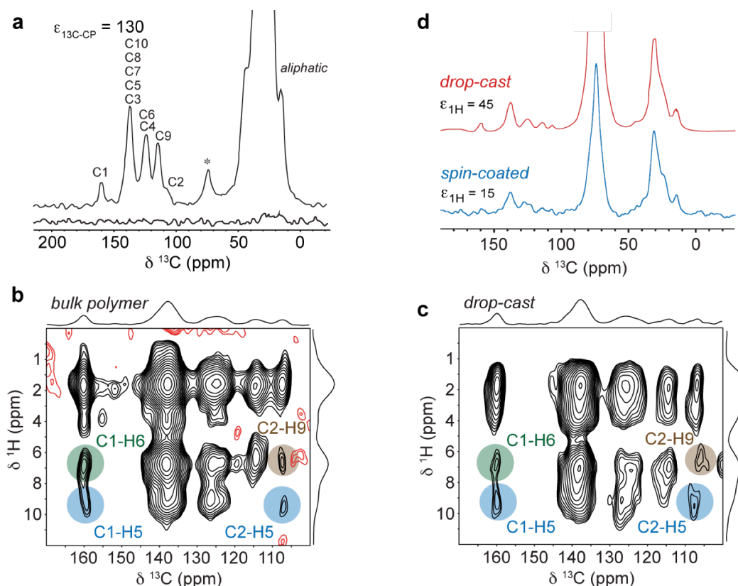
Figure 8. (a) DNP enhanced ^{13}\text{C} CPMAS NMR spectra of 1 mg of DPP-DTT bulk polymer recorded at 9.4 T and a MAS frequency of 11 kHz using a 16 mM TEKPol / TCE- d_2 polarizing solution. The spectra were recorded either with (upper spectrum) or without (lower spectrum) microwave irradiation at 263 GHz to induce DNP transfer. (b) DNP-enhanced ^1\text{H} - ^{13}\text{C} HETCOR spectra of DPP-DTT bulk polymer and (c) drop-cast film recorded using protonated TCE polarizing solution and eDUMBO-1 _{22} homonuclear ^1\text{H} dipolar decoupling 78 during t_1 . ^1\text{H} chemical shifts were corrected by applying a scaling factor of 0.57. (d) ^{13}\text{C} DNP-CPMAS NMR spectra of drop cast (red) and spin-coated (blue) films of DPP-DTT. Total experimental times were (a) 1.1 hours, (b) 6.4 hours, (c) 24 hours and (d) 1.4 hours (drop-cast) and 20 hours (spin-coated).
