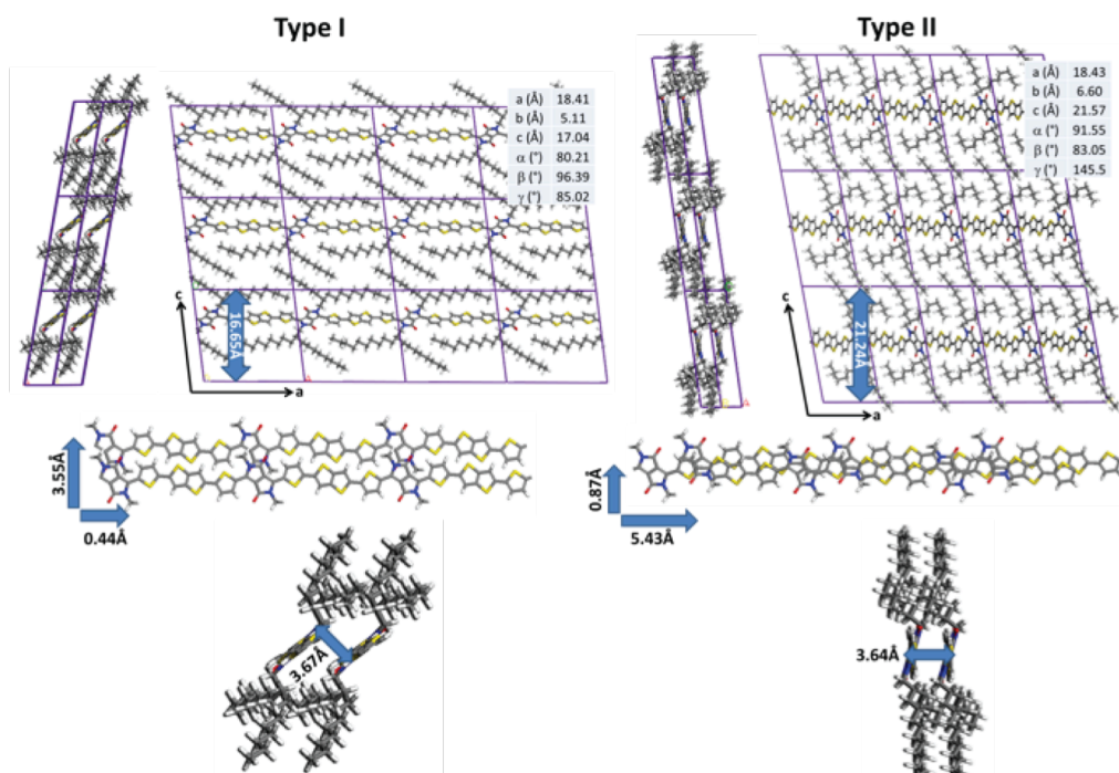
Figure 3. Representation of the molecular mechanics most stable DPP-DTT type I and type II structures with their cell parameters (top). Representation of the characteristic structural parameters of both conformers (shifts along the short and long polymer axes (center) and \pi -stacking distance (bottom)).
