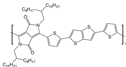
Figure 1. Chemical structure of diketopyrrolo-pyrrole-dithienylthieno[3,2-b]thiophene (DPP-DTT).
