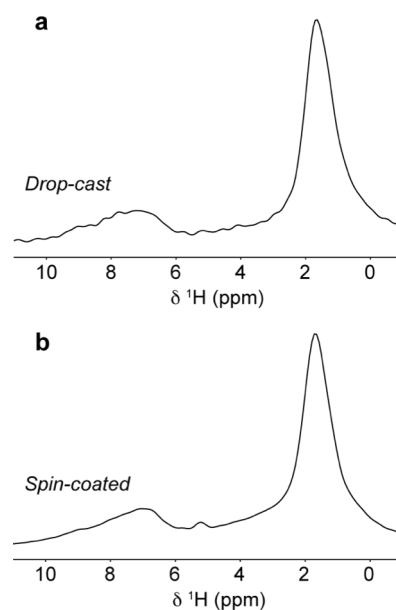
Figure 7. ^1\text{H} MAS NMR spectra of (a) drop-cast and (b) spin-coated films of DPP-DDT on crushed glass substrates recorded at 18.8 T and a MAS frequency of 60 kHz.
