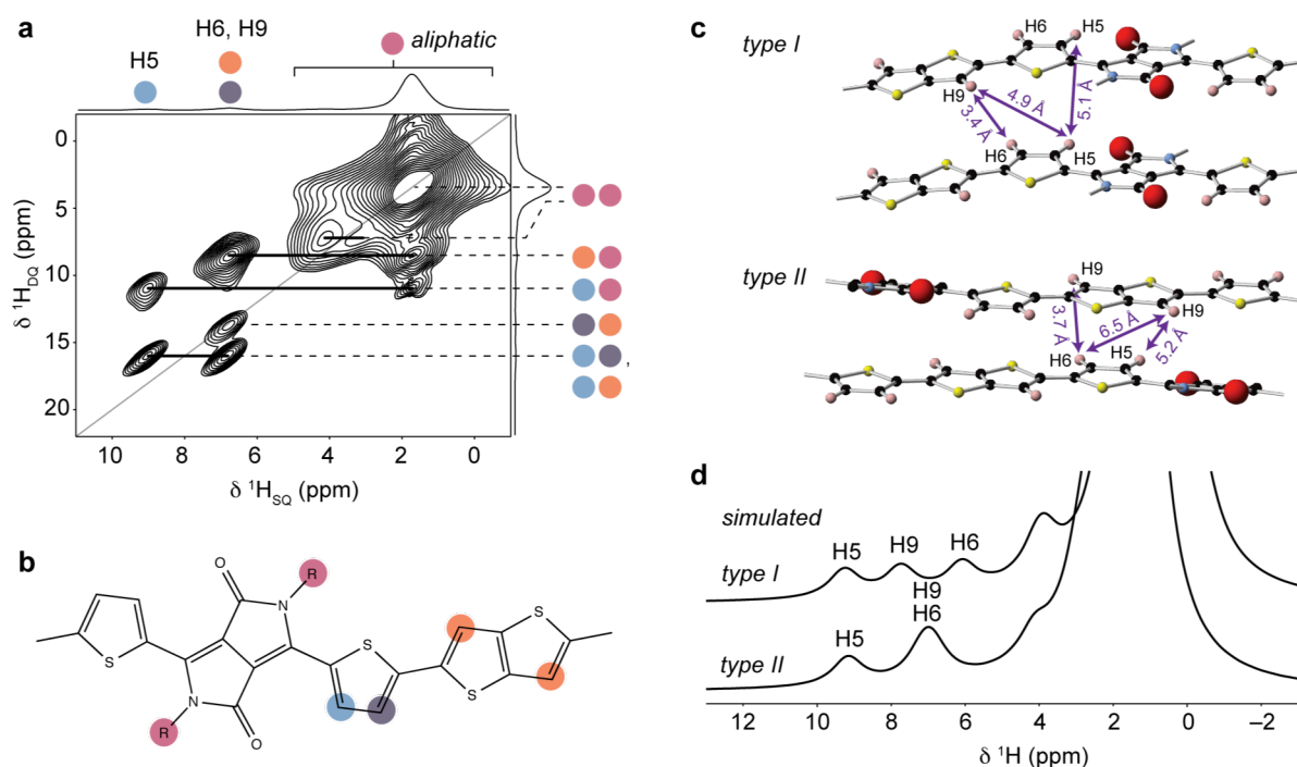
Figure 5. (a) ^1\text{H} DQ-SQ MAS NMR spectrum of DPP-DTT bulk polymer recorded at 18.8 T and a MAS frequency of 60 kHz, using the BABA pulse sequence 76 with a recoupling time of two rotor periods. (b) Schematic structure of the DPP-DTT repeat unit showing the labeling scheme for peak assignments in (a). (c) Sections of the MD-simulated type I and type II structures with relevant intermolecular H-H distances labeled. (d) Simulated ^1\text{H} MAS NMR spectra based on periodic-DFT-calculated NMR parameters for the type II and type I structures.
