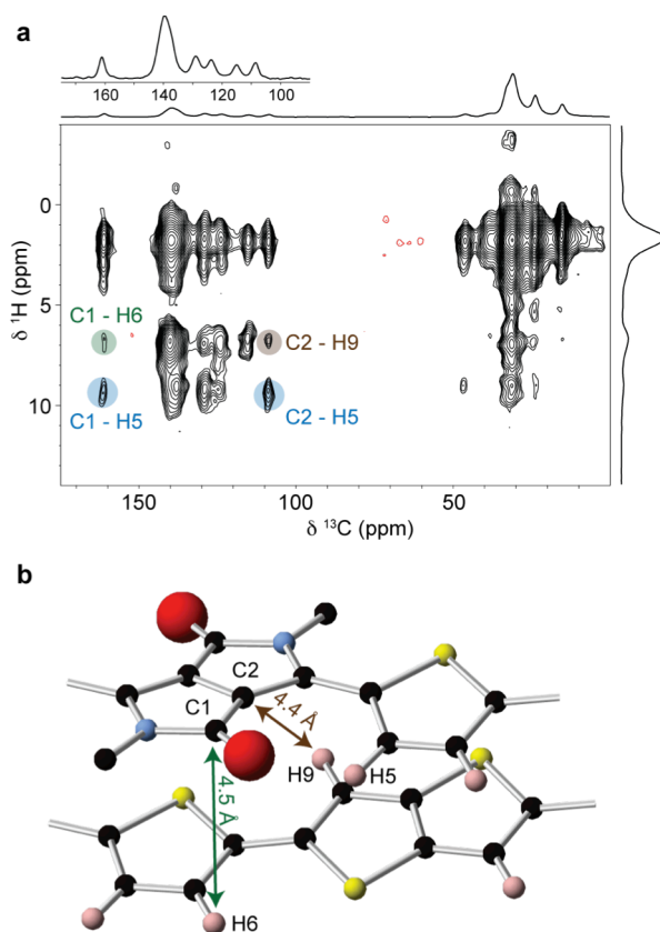
Figure 6. (a) ^1\text{H} - ^{13}\text{C} HETCOR NMR spectrum of 15 mg of DPP-DDT bulk polymer recorded at a magnetic field strength of 9.4 T and MAS frequency of 12.5 kHz in a total experimental time of 64 hours. (b) Section of the MD-simulated type II structure showing the close intermolecular proximity between carbons C1 and C2 on the DPP unit and aromatic protons on the neighbouring molecule.
