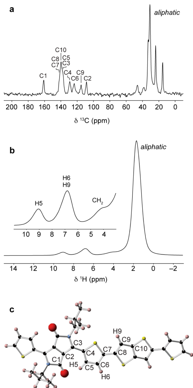
Figure 4. (a) ^1\text{H} - ^{13}\text{C} CPMAS and (b) ^1\text{H} MAS NMR spectra of DPP-DTT bulk polymer. Spectra were recorded at magnetic field strengths of (a) 9.4 and (b) 18.8 T, and MAS frequencies of (a) 12.5 and (b) 60 kHz. (c) DFT-optimized polymer fragment used for NMR chemical shift calculations.
